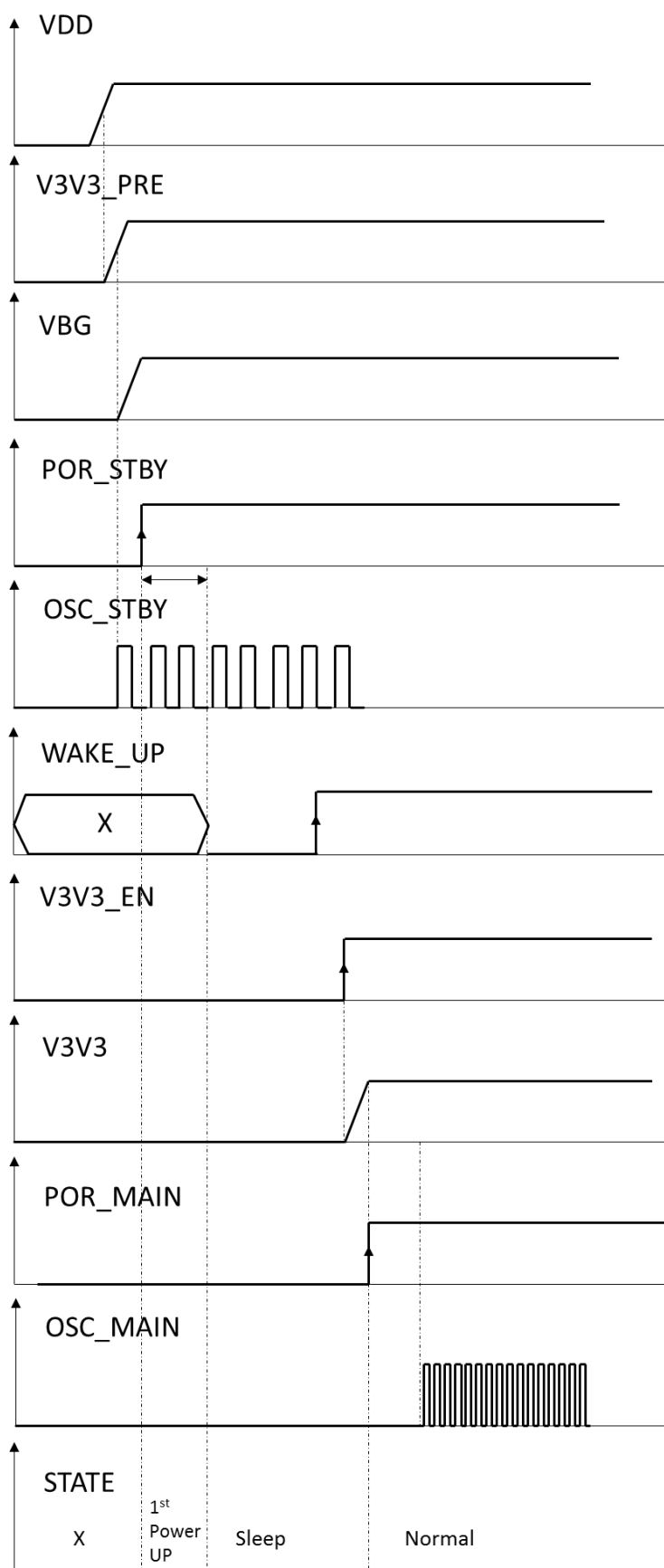
Figure 13. First power up sequence
