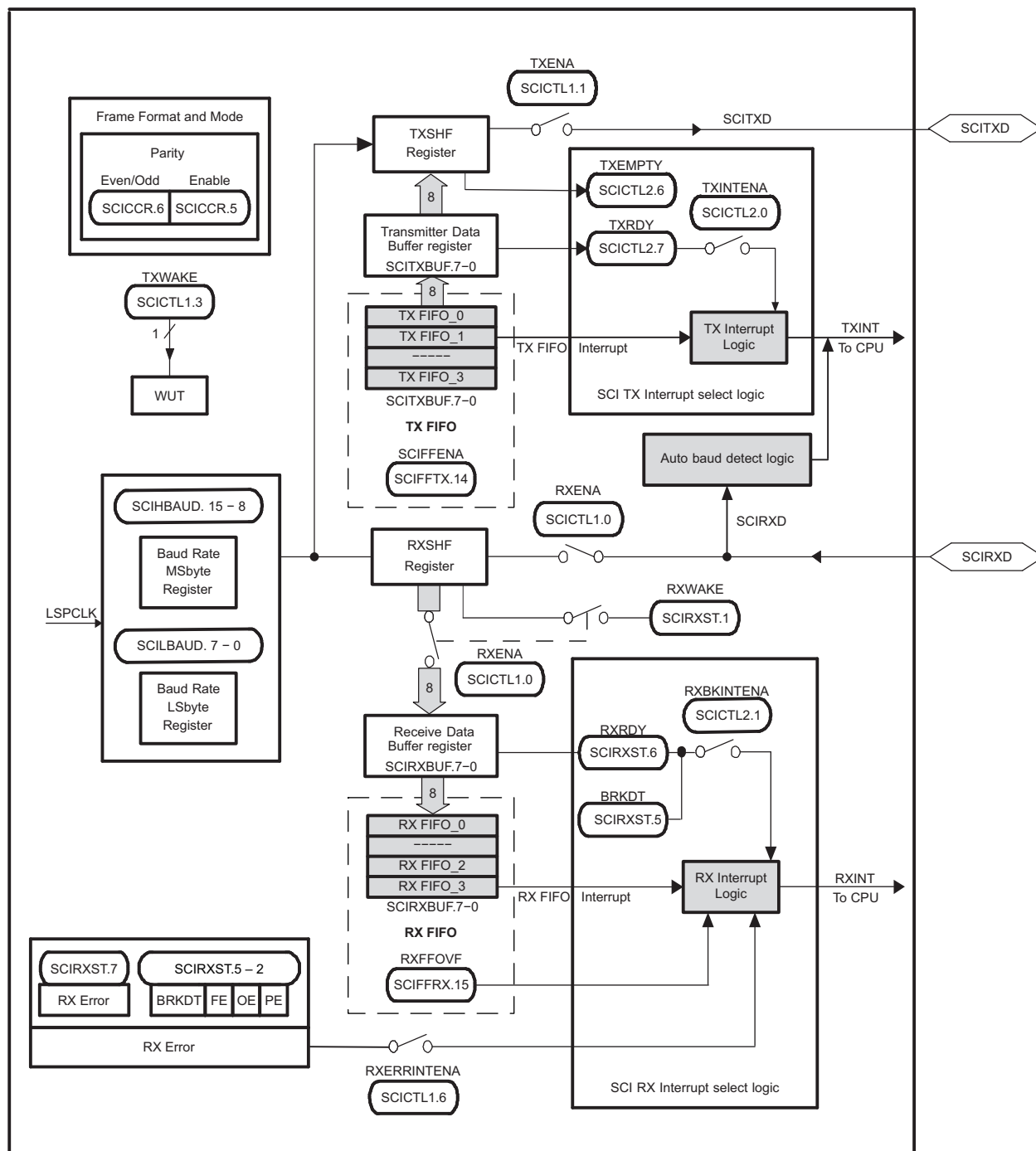
Figure 6-37. Serial Communications Interface (SCI) Module Block Diagram
