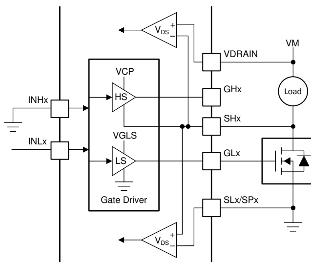
图 26. Single Low-Side Driver
