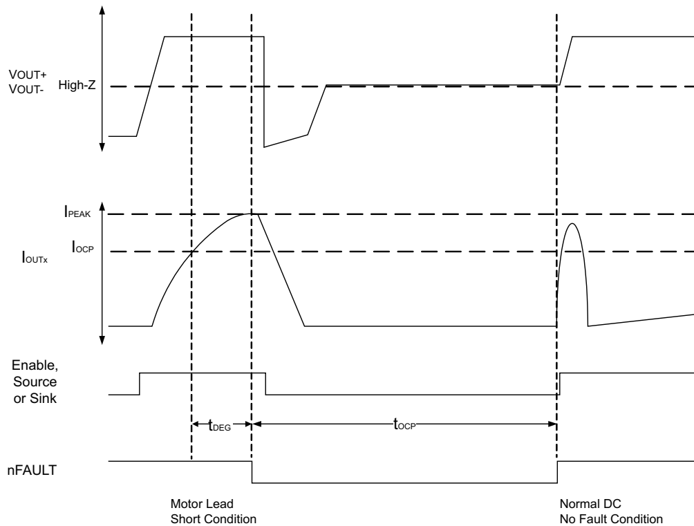
Figure 6. Overcurrent Threshold
