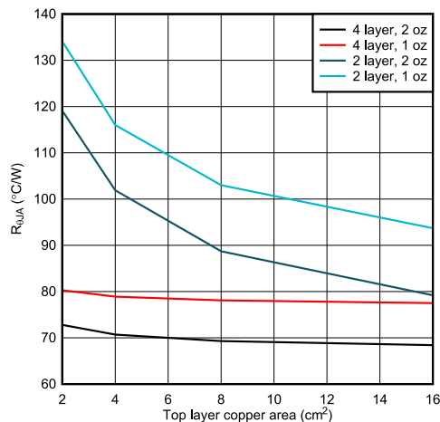
Figure 9-27. WSON, PCB junction-to-ambient thermal resistance vs copper area
