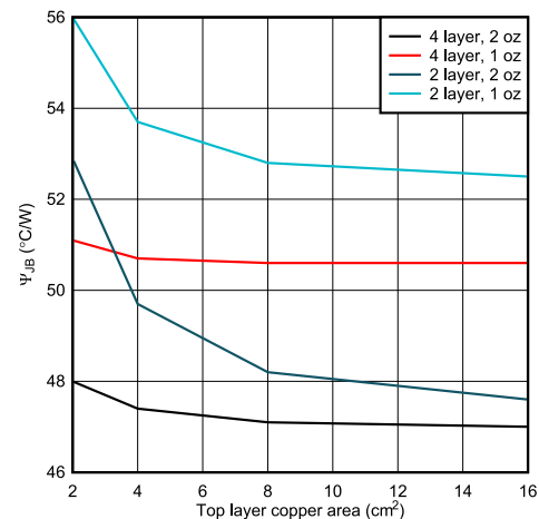
Figure 9-28. WSON, junction-to-board characterization parameter vs copper area
