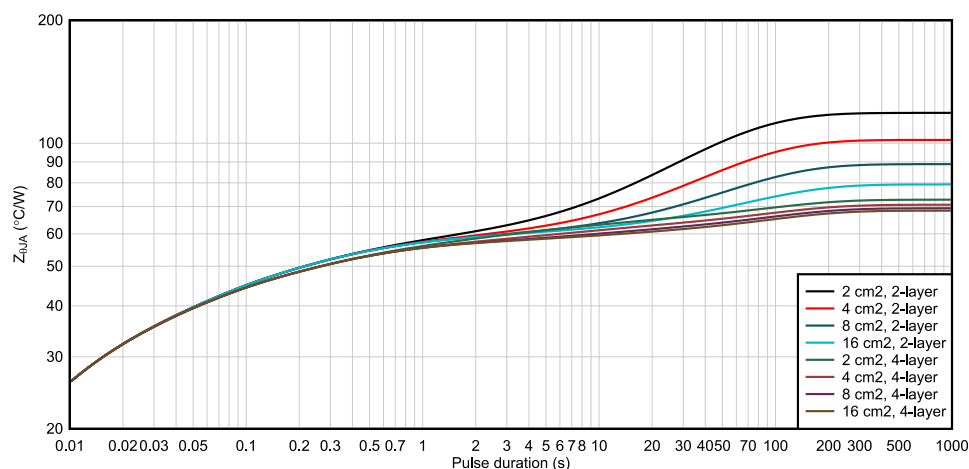
Figure 9-30. WSON package Junction-to-ambient thermal impedance for 2-oz copper layouts
