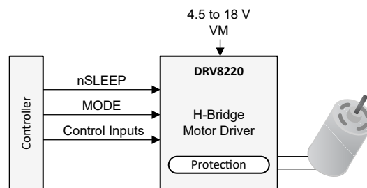
Simplified Schematic
