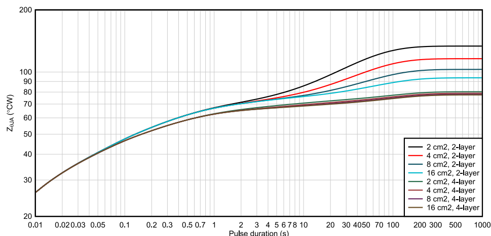
Figure 9-29. WSON package junction-to-ambient thermal impedance for 1-oz copper layouts
