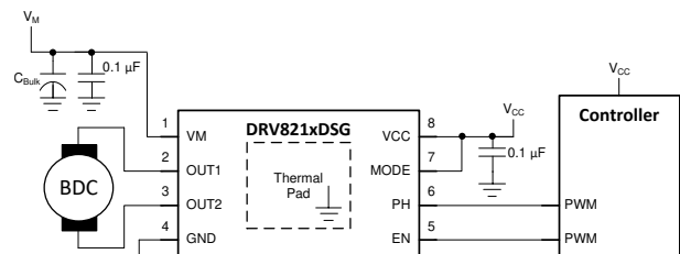
Figure 9-2. PWM interface motor-driving application for DSG package
