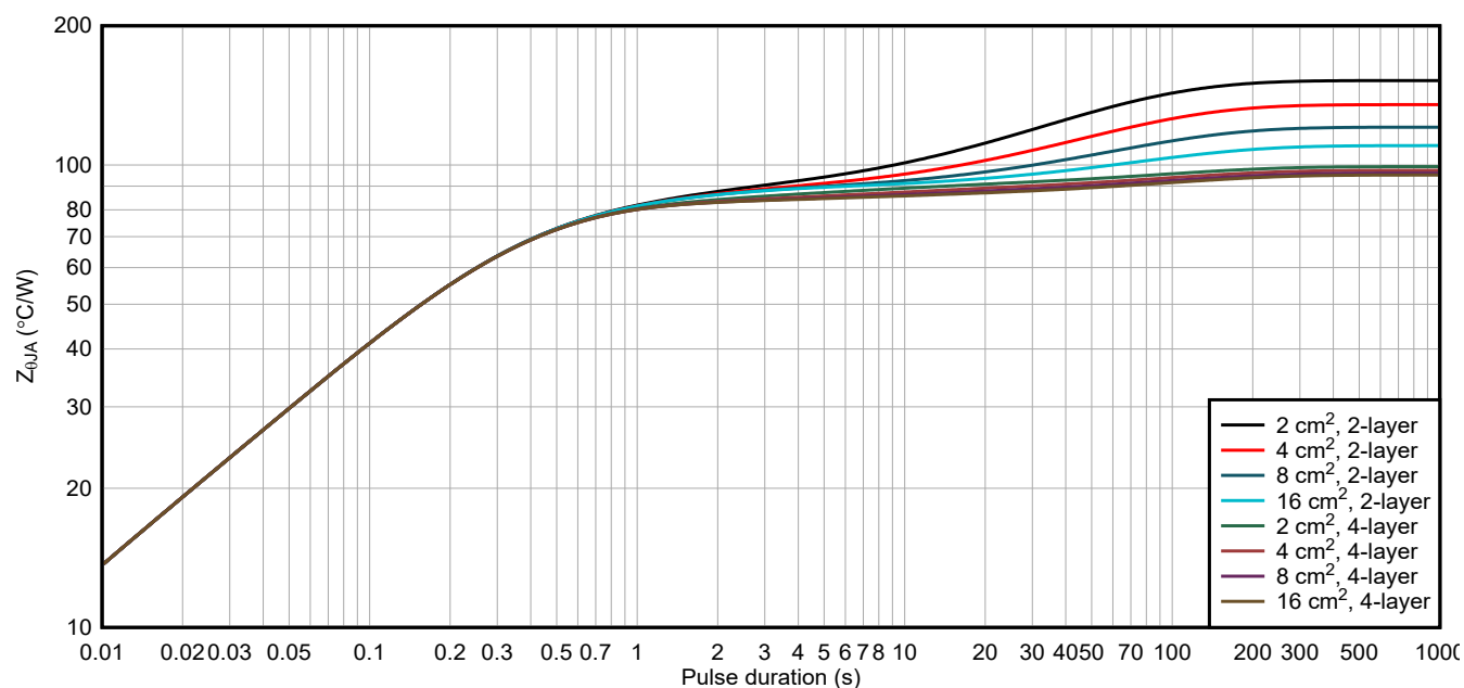
Figure 9-38. DRL package junction-to-ambient thermal impedance for 2-oz copper layouts
