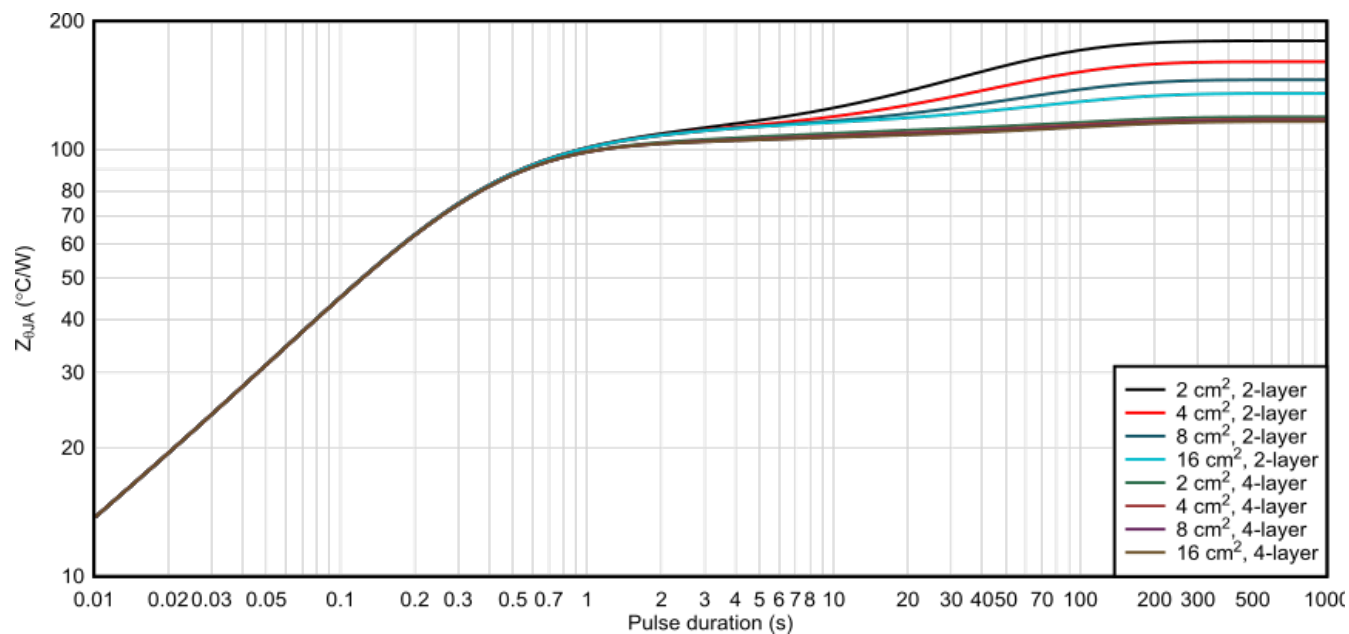
Figure 9-37. DRL package junction-to-ambient thermal impedance for 1-oz copper layouts
