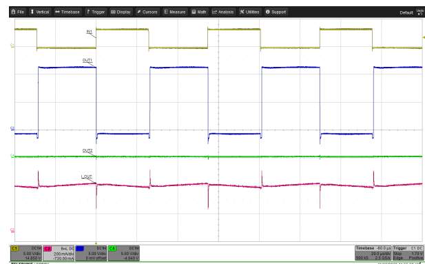
A. Channel 1 = IN1 Channel 2 = Motor Current Channel 3 = OUT1 Channel 4 = OUT2
