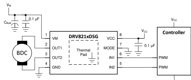
Figure 9-2. PWM interface motor-driving application for DSG package
