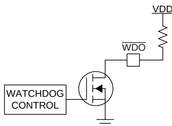
图 12. \overline{\text{WDO}} Open-Drain Configuration
