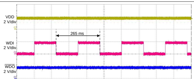
图 17. Typical WDI Signal
