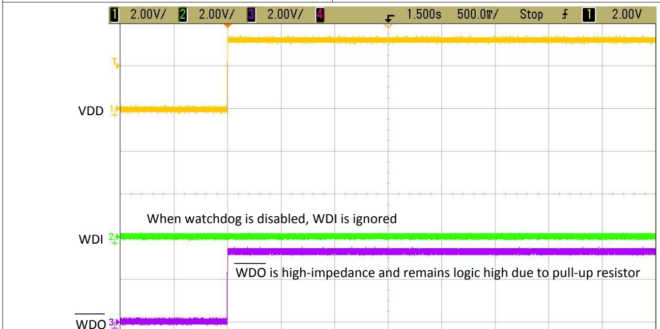
图 18. Watchdog Disabled With Missing WDI Pulse
