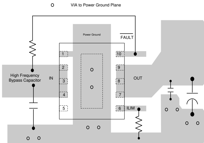
图 11-1. TPS2559 Board Layout
