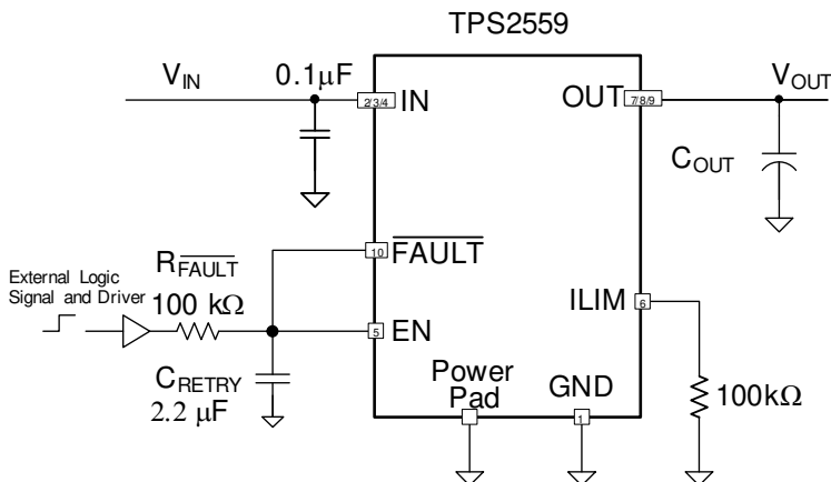
图 9-4. Auto-Retry Circuit with External EN Signal
