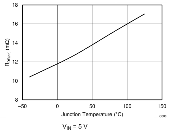
图 7-10. Input/Output Resistance ( R_{DS(on)} ) vs Temperature
