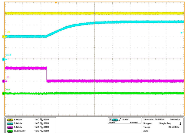
Figure 8-13. LM73100 Reverse Current Protection During 20-V Voltage Ramp at Output
