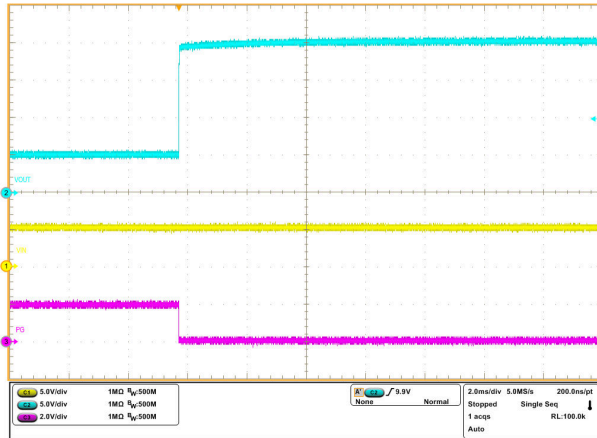
Figure 8-12. LM73100 Reverse Current Protection During 20-V Hot-Plug at Output
