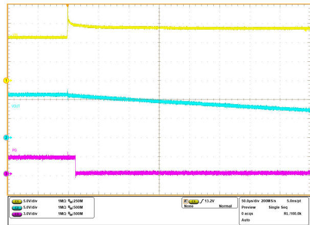
Figure 8-5. Overvoltage protection
