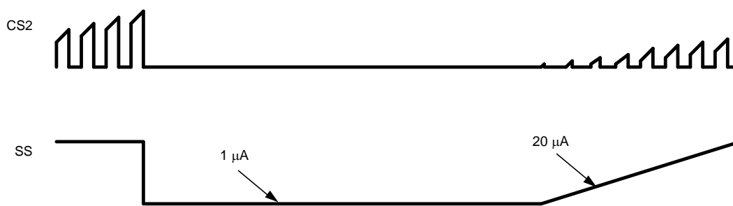
Figure 12. Current Limit
