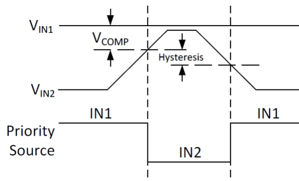
图 19. VCOMP Priority Source Selection
