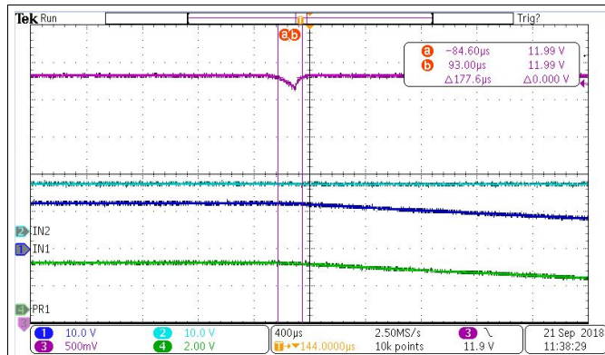
图 32. Seamless Switchover Between Two 12-V Supplies
