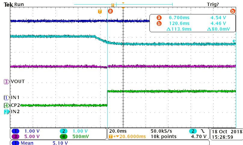
图 37. Switchover from IN2 to IN1
