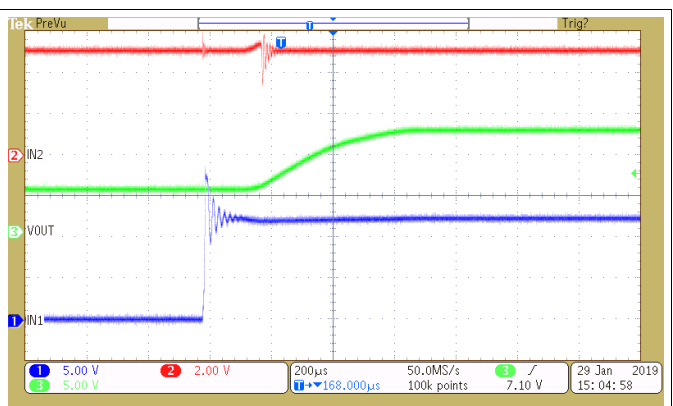
图 41. TPS2121 Hotplug Event with TVS1800
