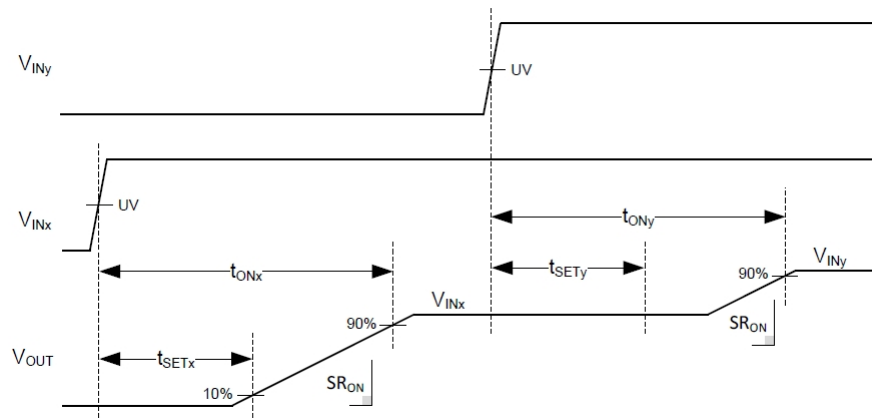
图 12. Settling and Soft Start Timing
