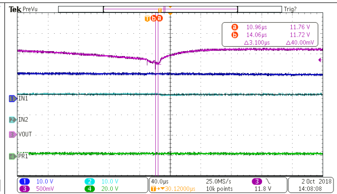
图 33. Fast Switchover Demonstration
