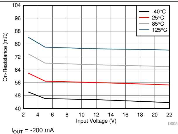
图 5. TPS2121 On-Resistance vs Input Voltage
