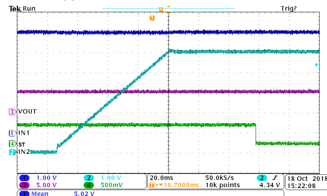
图 35. Switchover from IN1 to IN2
