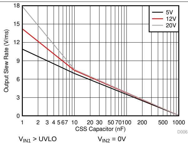
图 6. Output Slew Rate vs CSS Capacitor
