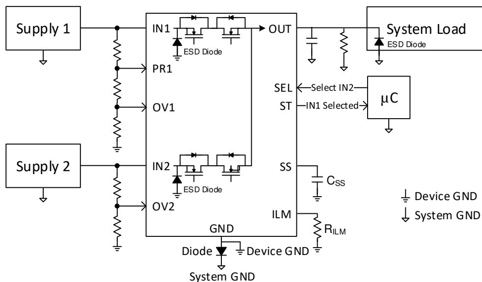
图 38. TPS212x Reverse Polarity Configuration
