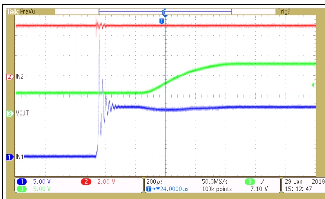
图 40. TPS2121 Hotplug Event without TVS
