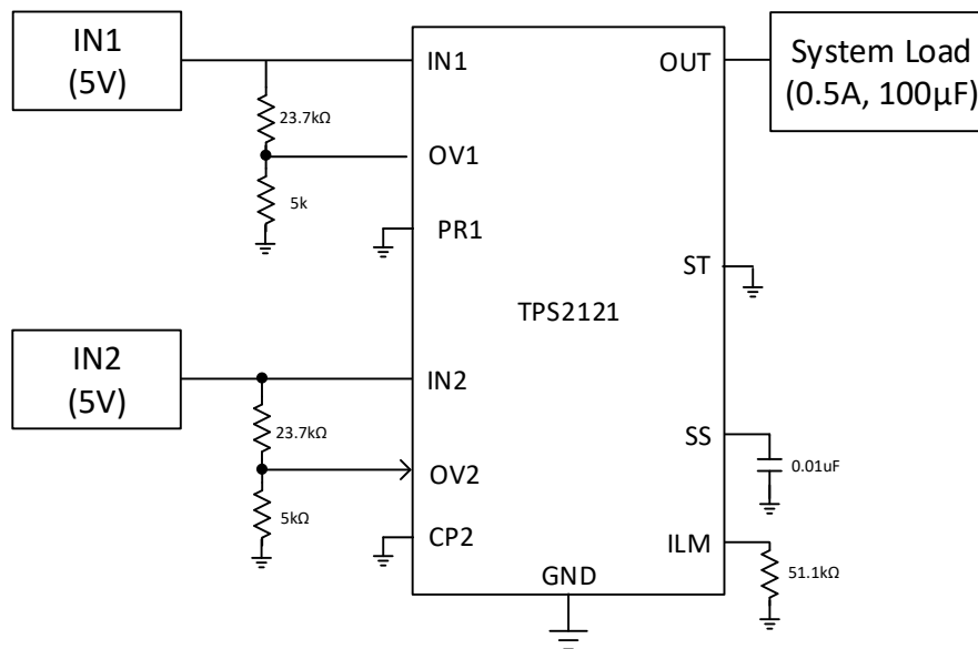
图 34. Highest Voltage Operation
