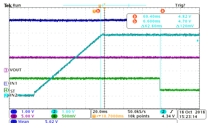
图 36. Timing from IN1 to IN2
