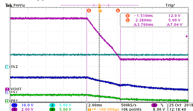
图 29. Automatic Switchover from IN1 to IN2
