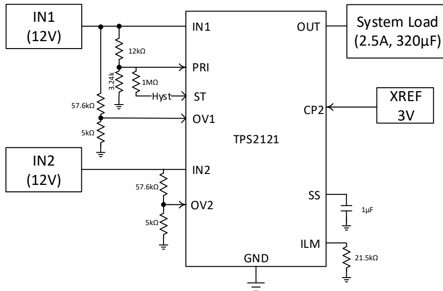
图 31. Automatic Switchover Between Two 12-V Supplies
