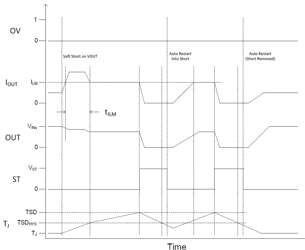
图 13. Current Limiting Behavior
