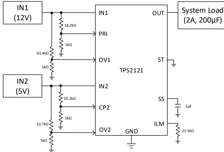
图 28. Automatic Switchover Between 12 V and 5 V
