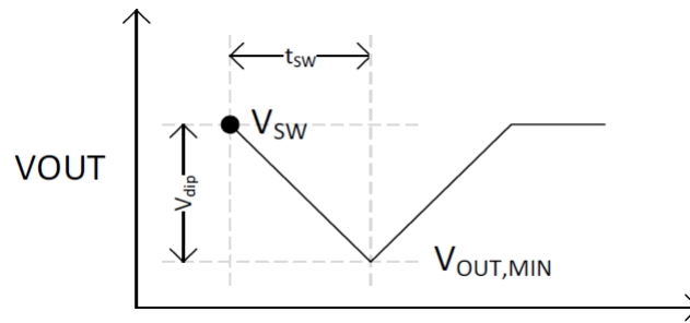
图 16. Minimum Output Voltage During Fast Switchover
