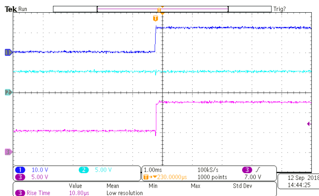
图 30. Automatic Switchover from IN2 to IN1
