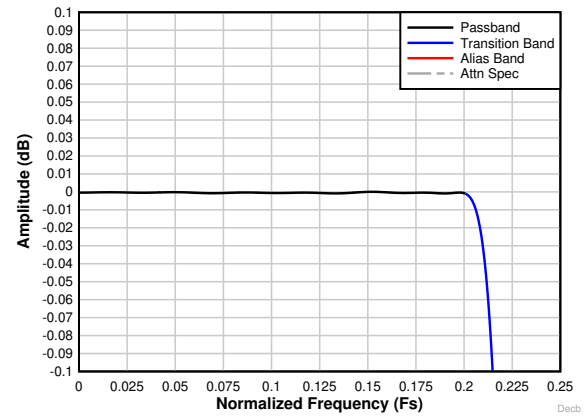
图 8-27. Decimation by 2 complex passband ripple response
