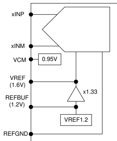
图 8-15. Different voltage reference options for ADC358x
