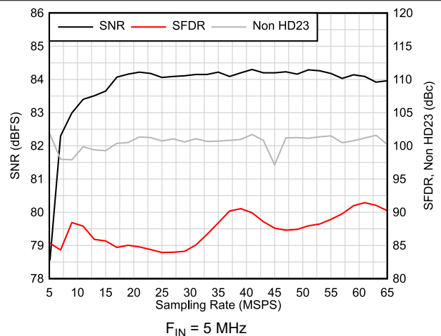
图 6-14. AC Performance vs Sampling Rate
