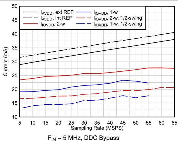
图 6-24. Current vs Sampling Rate
