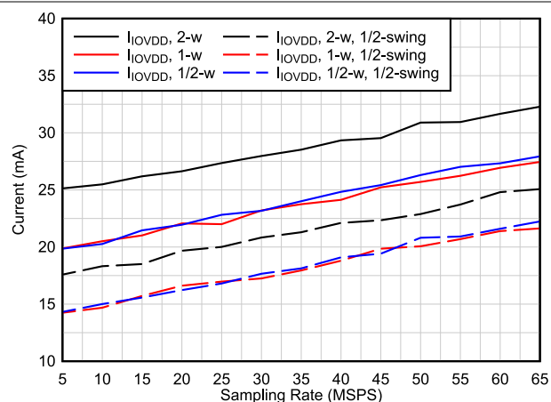
图 6-26. I_{IOVDD} Current vs Output Interface
