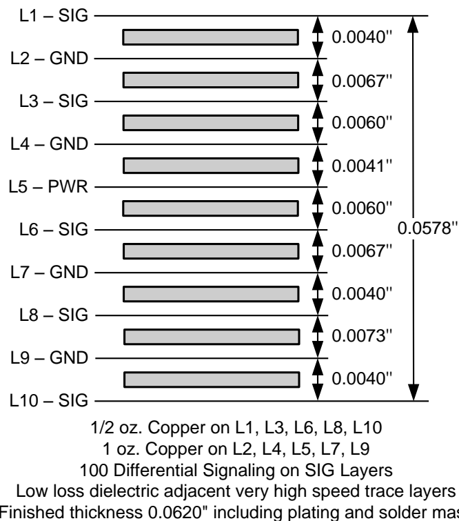
图 117. ADC12J1600 and ADC12J2700 Typical Stackup — 10 Layer Board
