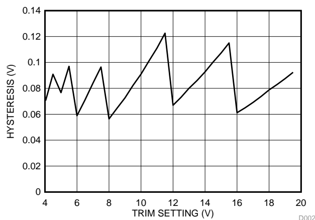
Figure 3. Hysteresis on V_{\text{LOW\_BAT}} and V_{\text{UVLO}}
