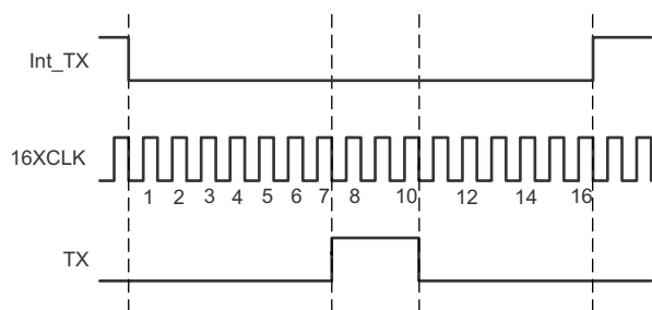
图 37. IrDA-SIR Decoding Scheme – Detailed Timing Diagram
