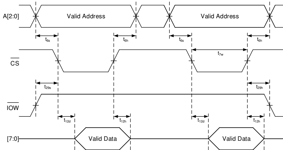
图 5. General Read Timing ( \overline{\text{IOW}} Only Mode, \text{MODE} = \text{GND} )
