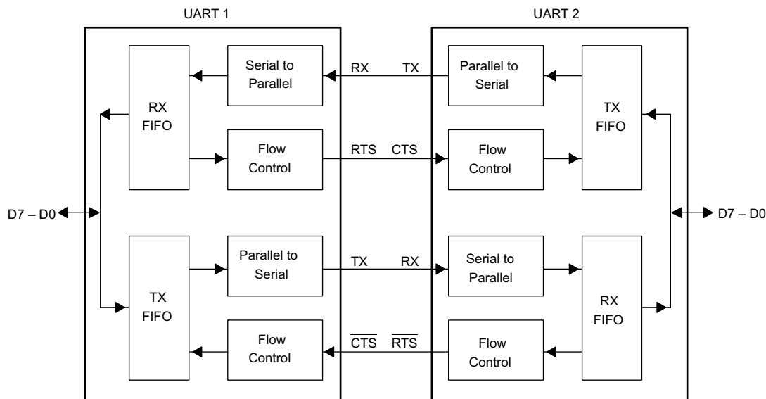
图 22. Autoflow Control (Auto- \overline{\text{RTS}} and Auto- \overline{\text{CTS}} ) Example
