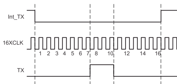
图 35. IrDA-SIR Encoding Scheme – Detailed Timing Diagram
