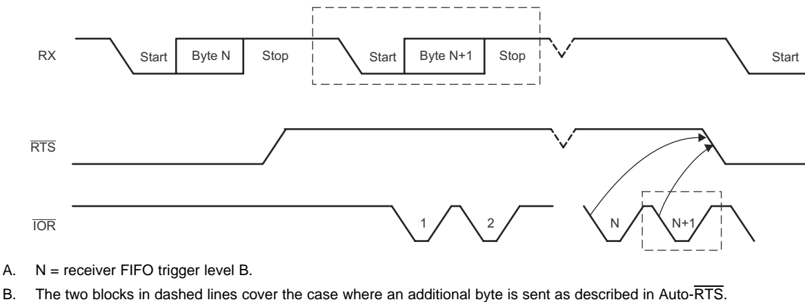
图 20. \overline{\text{RTS}} Functional Timing
