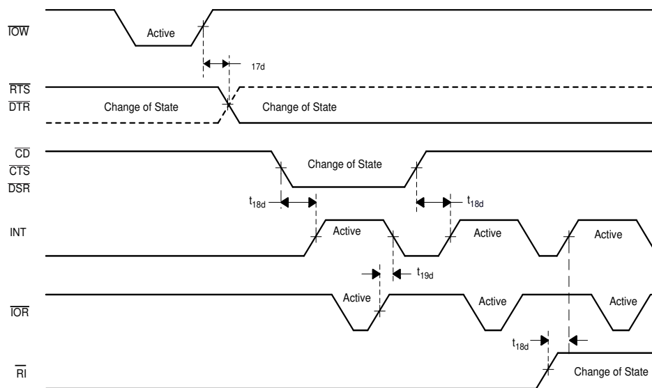
图 6. Modem or Output Timing ( \overline{\text{IOR}} and \overline{\text{IOW}} Mode, \text{MODE} = \text{VCC} )
