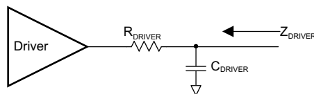
Figure 10. Z DRIVER Circuit
