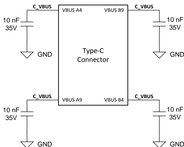
Figure 35. Type-C Connector VBUS Capacitors
