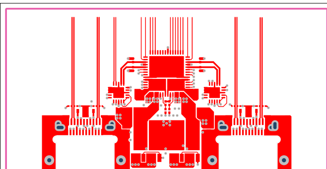
Figure 65. SSTXRX1 Layer
