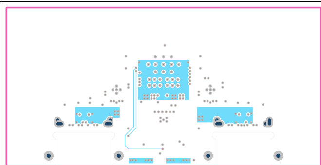
Figure 67. Power 1 Layer
