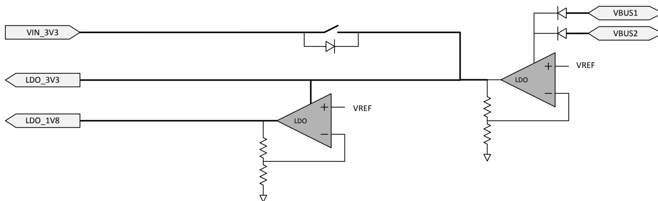
Figure 12. Power Supplies
