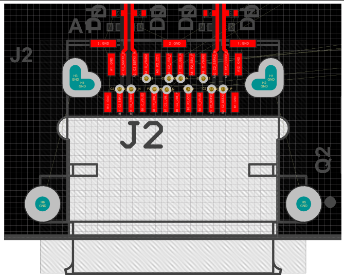
Figure 50. Type-C Connector SSTXRX Top Layer
