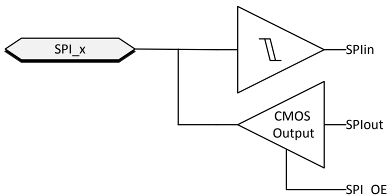
Figure 24. SPI buffer
