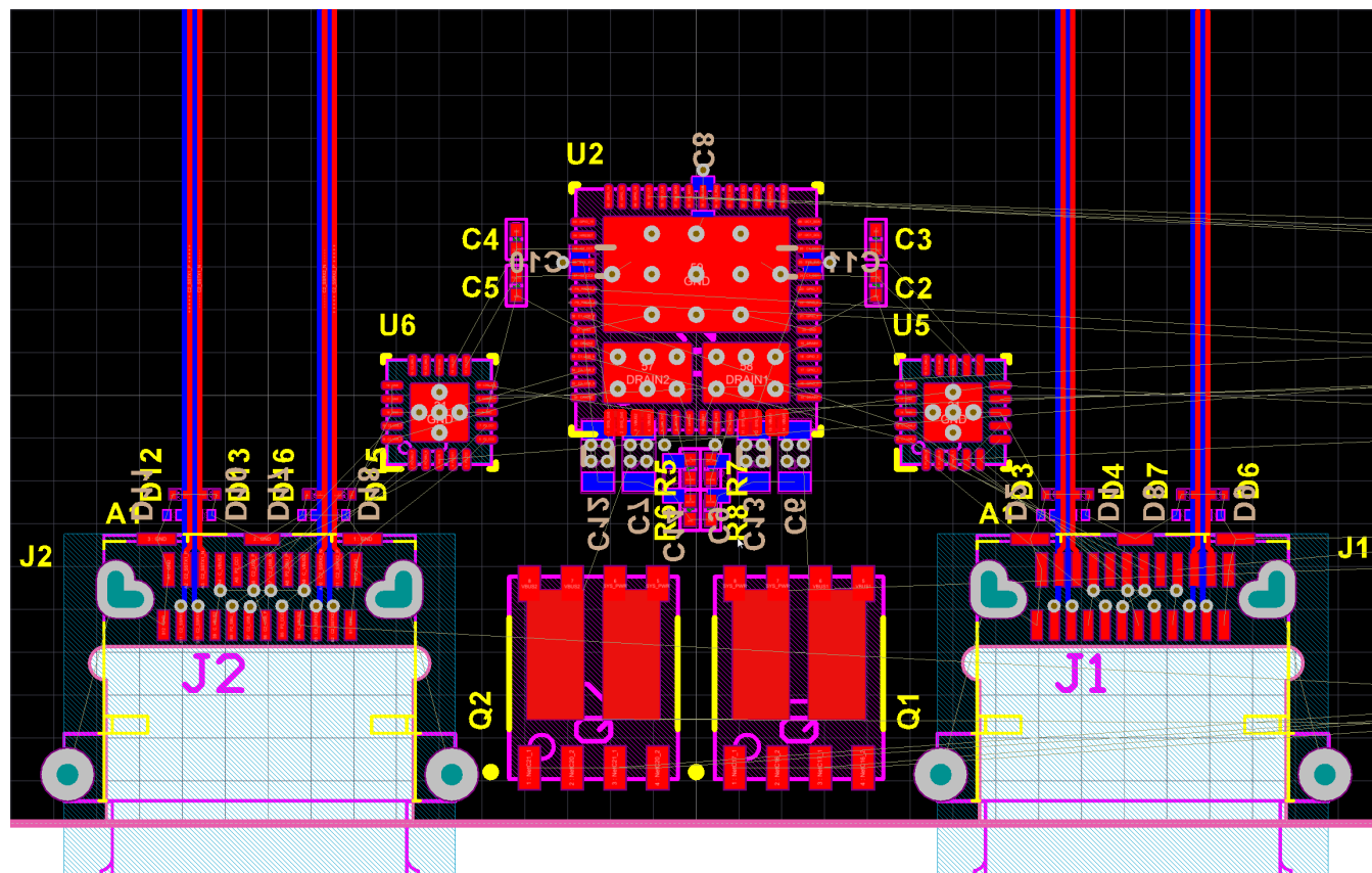
Figure 56. Protection Placement
