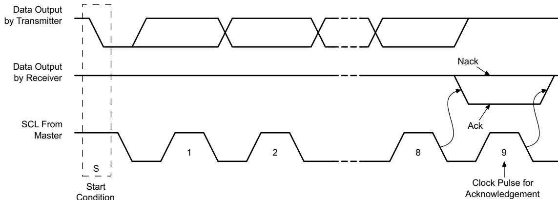
Figure 28. I²C Acknowledgment
