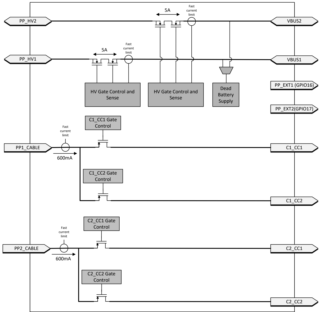
Figure 13. Port Power Switches
