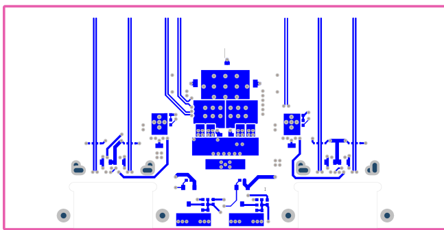
Figure 69. SSTXRX2 Layer
