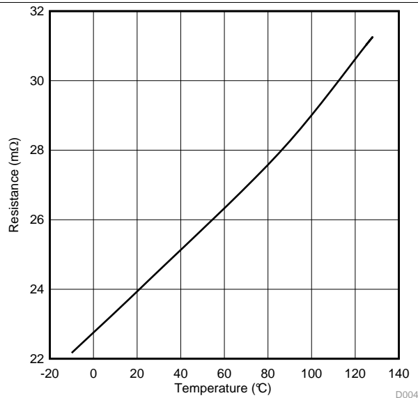
Figure 1. PPHVx Rdson vs Junction Temperature
