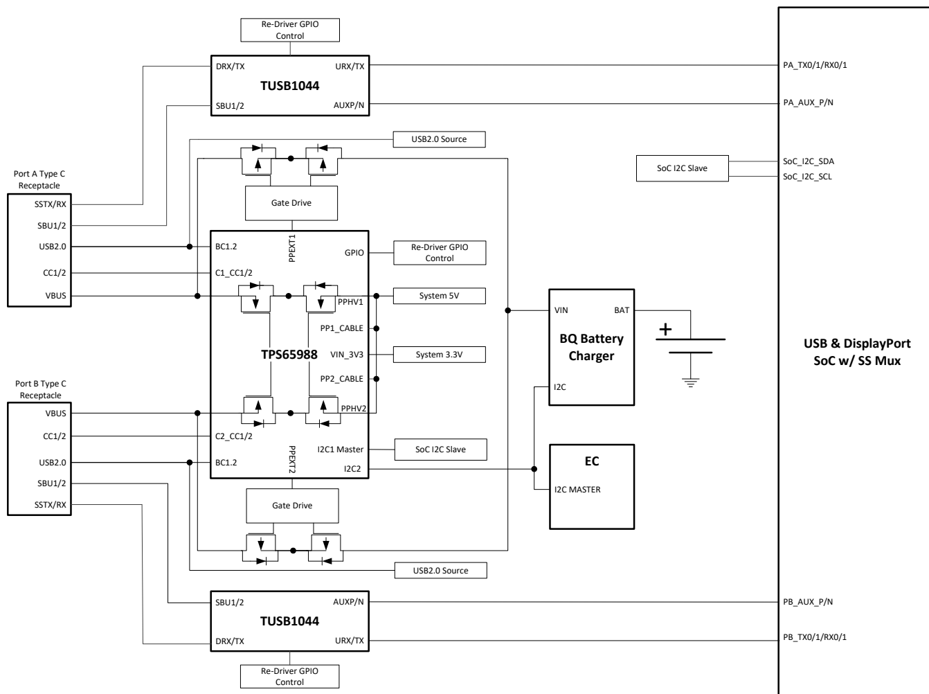
Figure 41. TPS65988 and SoC I2C w/ Re-Driver GPIO
