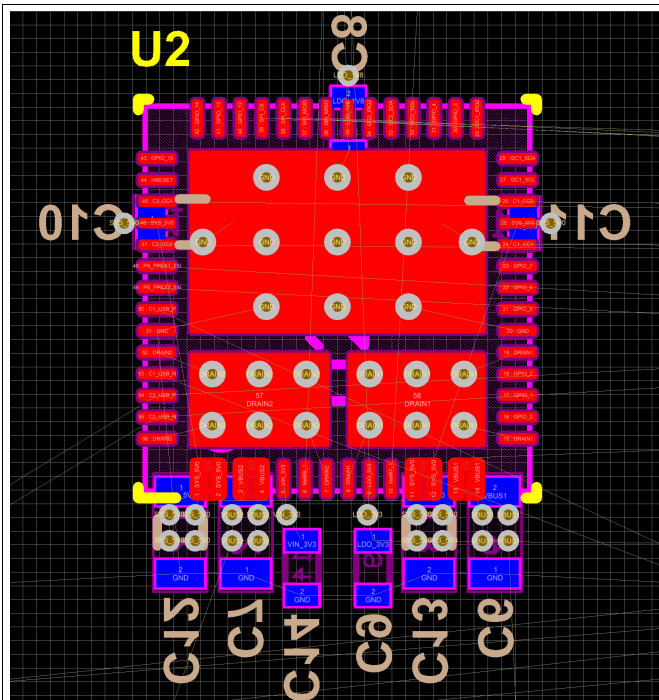
Figure 52. System Capacitors Placement Top/Bottom Layer
