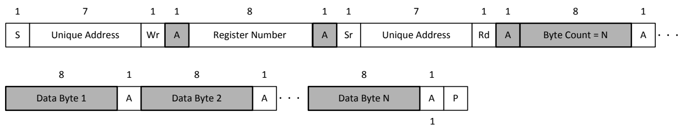
图 31. I 2 C Unique Address Read Register Protocol
