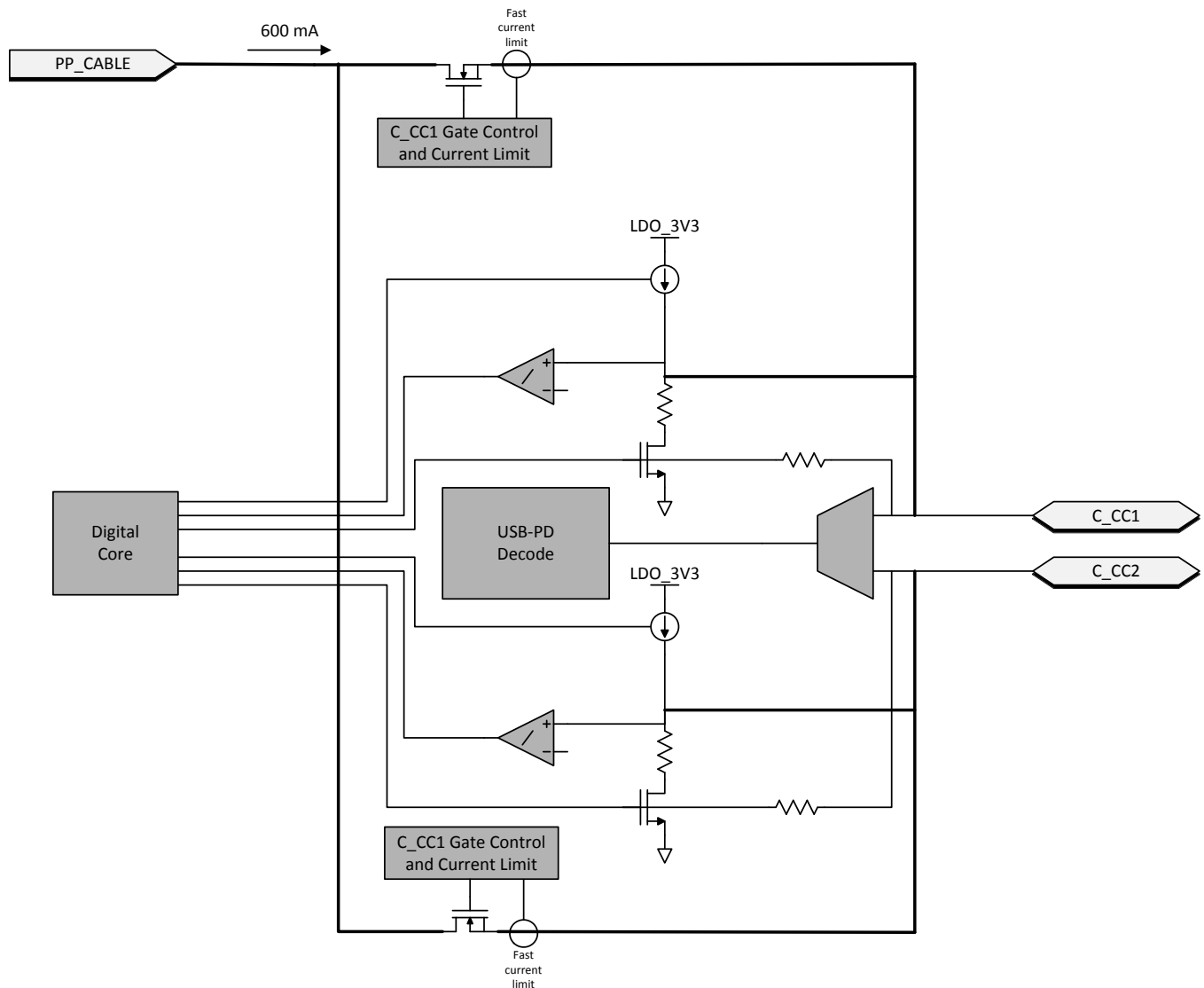
图 5. USB-PD Physical Layer, Simplified Plug and Orientation Detection Circuitry
