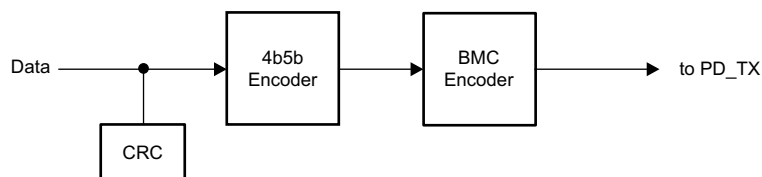
图 6. USB-PD Baseband Transmitter Block Diagram
