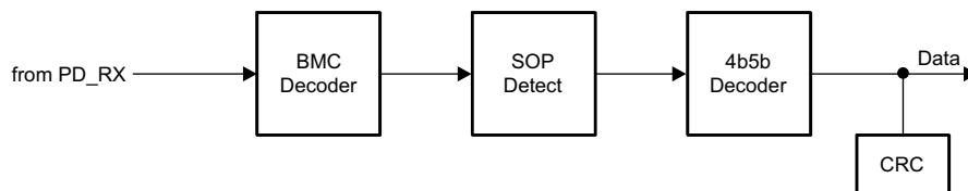
图 7. USB-PD Baseband Receiver Block Diagram
