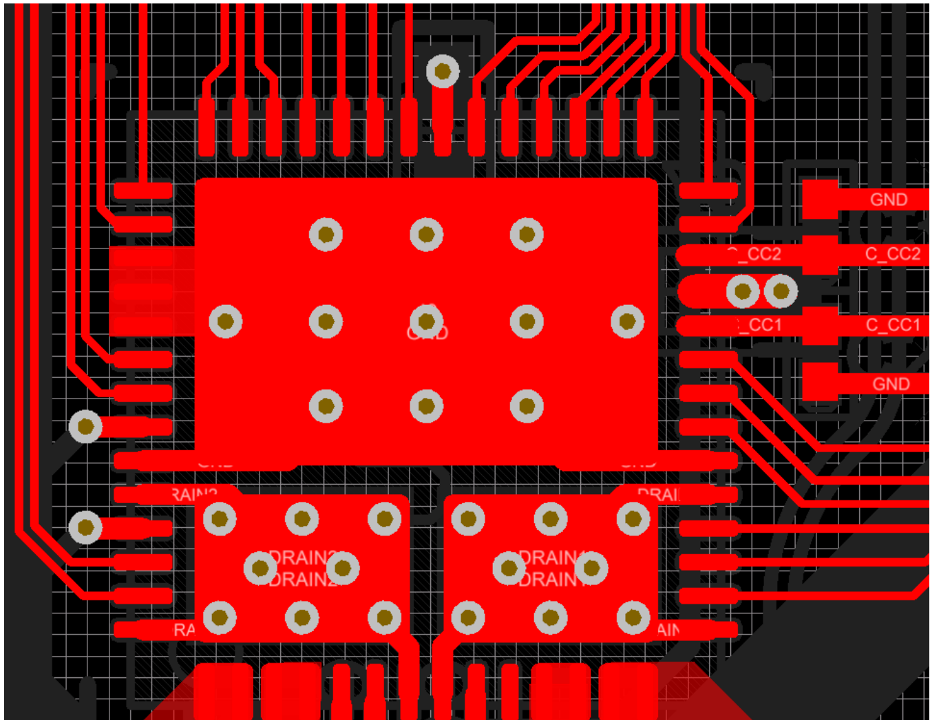
图 52. CC Routing and GPIO Fan-Out
