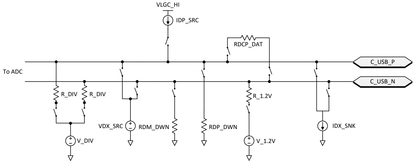
图 22. Battery Charger Detection and Advertisement
