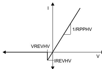
图 15. Comparator Mode (Source) Internal HV Switch I-V Curve
