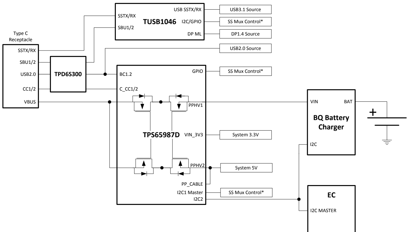
图 39. USB and DisplayPort Notebook Supporting PD Charging
