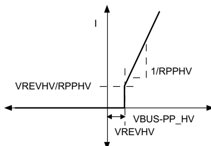
图 16. Ideal Diode Mode (Sink) Internal HV Switch I-V Curve
