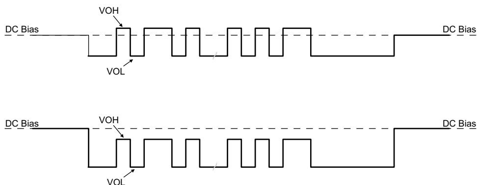
图 10. TX Driver Transmission with DC Bias
