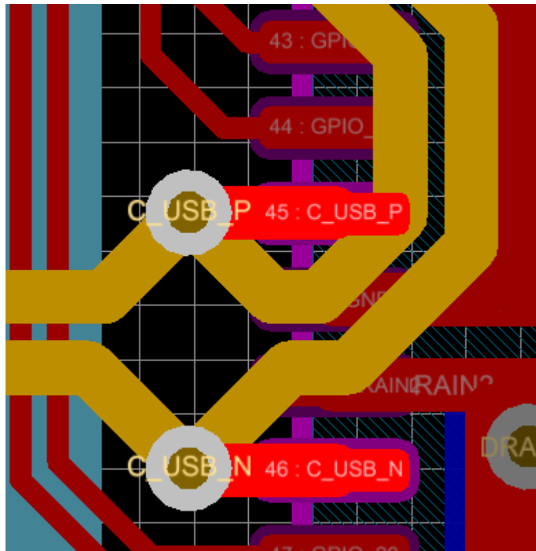
图 57. Via Connection for USB2
