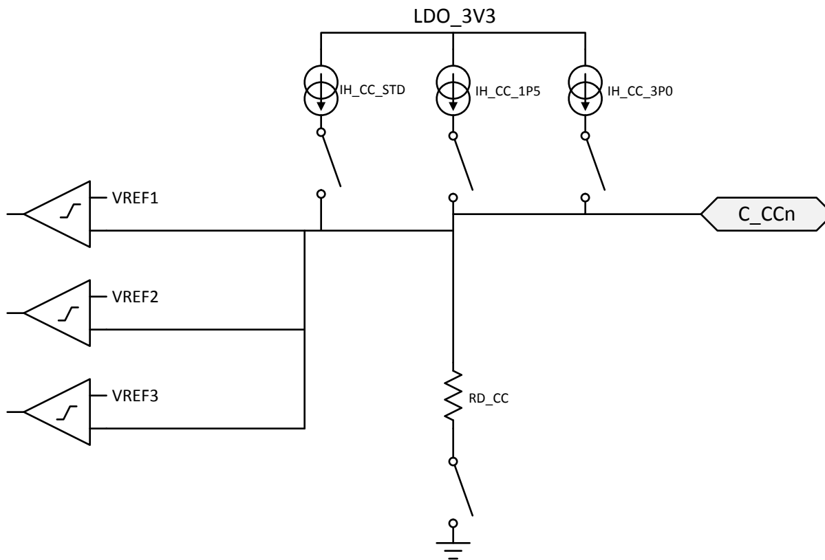
图 18. Plug and Orientation Detection Block
