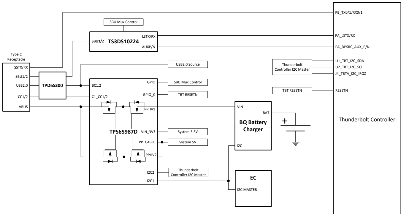
图 40. Thunderbolt Notebook Supporting PD Charging
