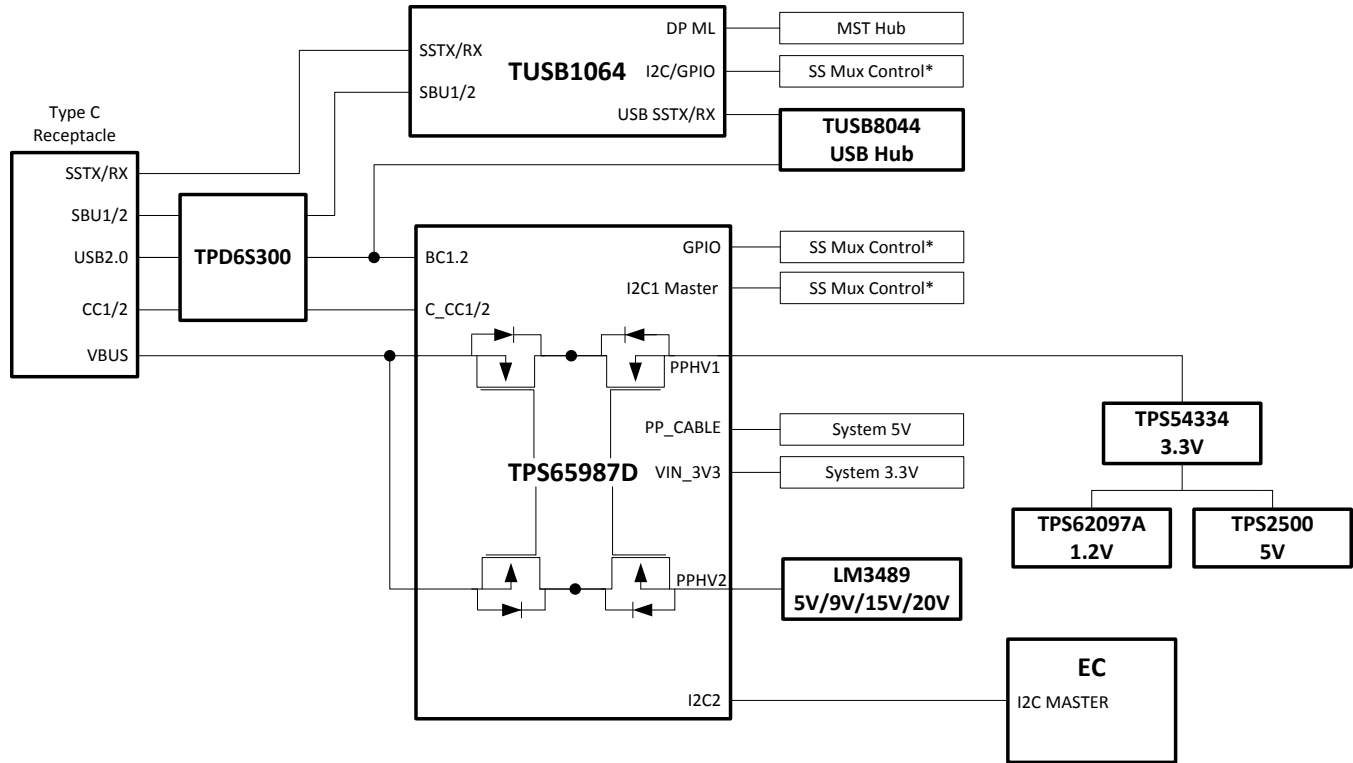
图 42. USB and DisplayPort Dock Block Diagram
