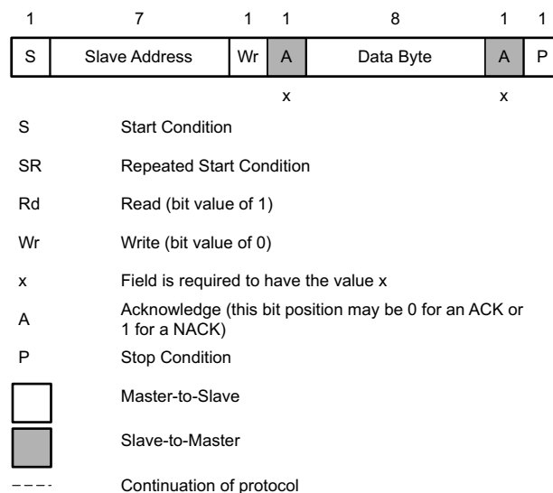
图 32. I 2 C Read/Write Protocol Key
