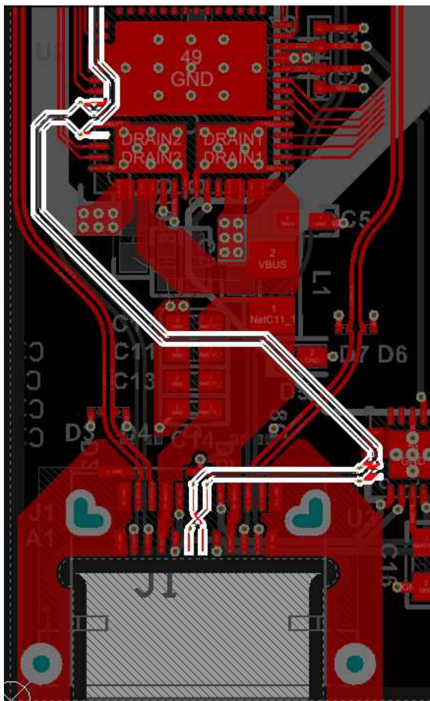
图 58. Complete USB2 Routing
