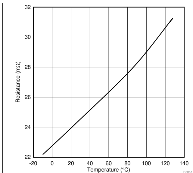
图 1. PPHVx Rdson vs Junction Temperature
