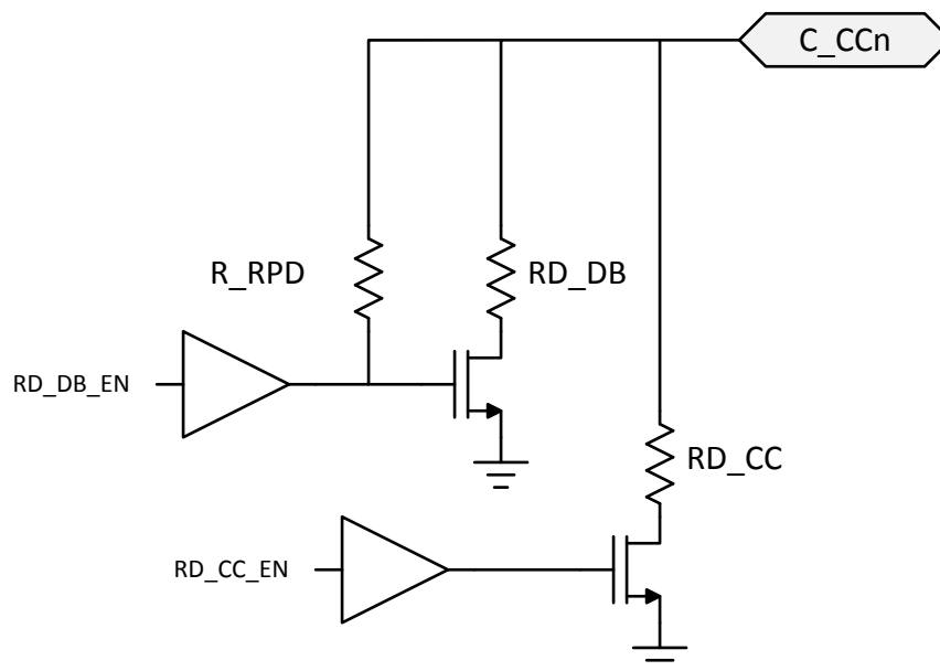
图 20. Dead Battery Pull-Down Resistor
