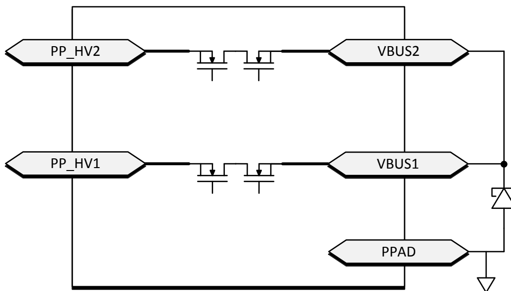
图 17. Schottky for Current Surge Protection
