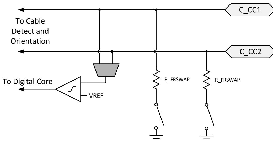
图 19. Fast Role Swap Detection and Signaling
