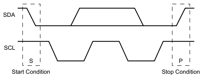
图 27. I 2 C Definition of Start and Stop Conditions
