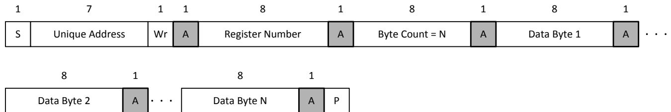
图 30. I 2 C Unique Address Write Register Protocol
