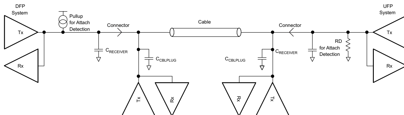
图 12. Example USB-PD Multi-Drop Configuration
