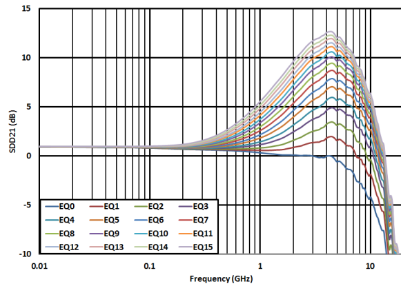
图 3. USB TX (UFP) EQ Settings Curves
