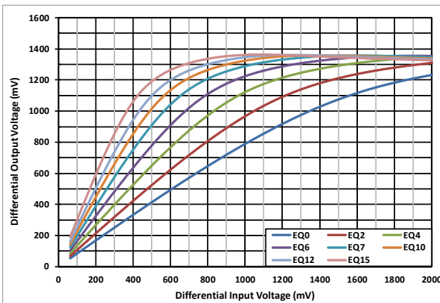
图 3. USB TX (UFP) EQ Settings Curves
