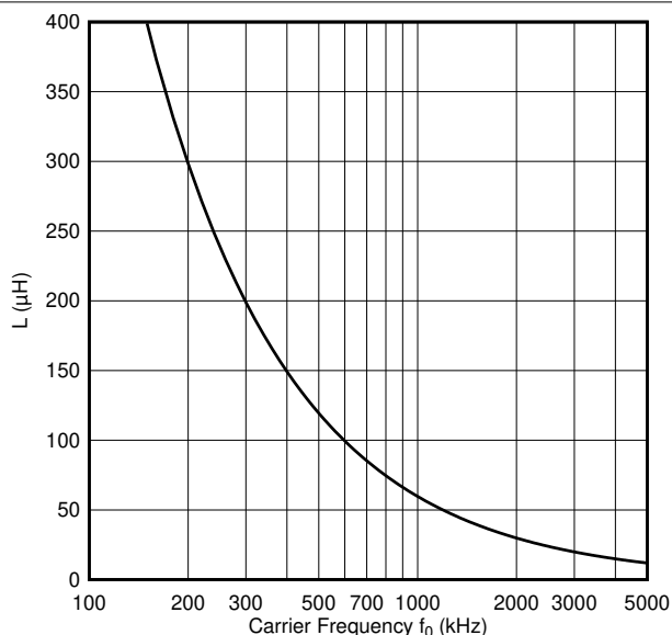
图 9-2. Inductor selection (select values above the line)
