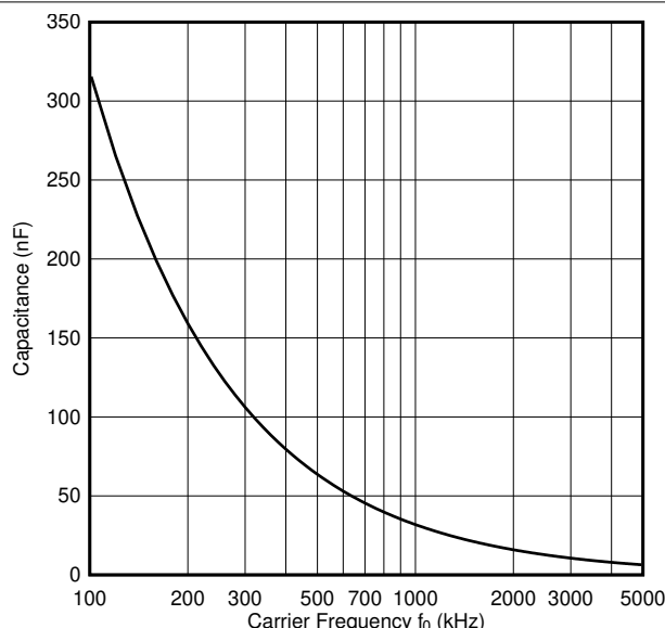
图 9-3. Capacitor selection (select values above the line)
