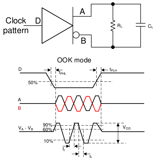
图 7-4. Measurement of Driver Switching Characteristics
