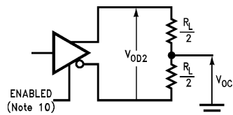
Figure 7. Differential and Common Mode Output Voltage
