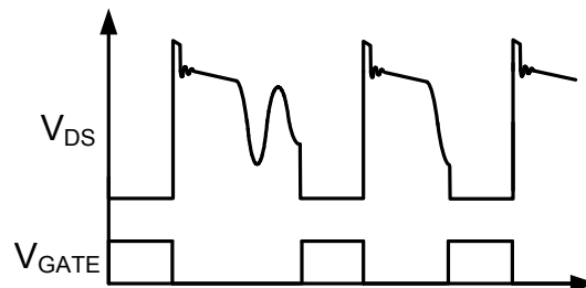
Figure 16. Valley-Skipping Mode
