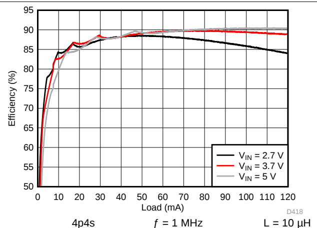
图 166. Backlight System Efficiency
