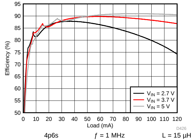
图 176. Backlight System Efficiency
