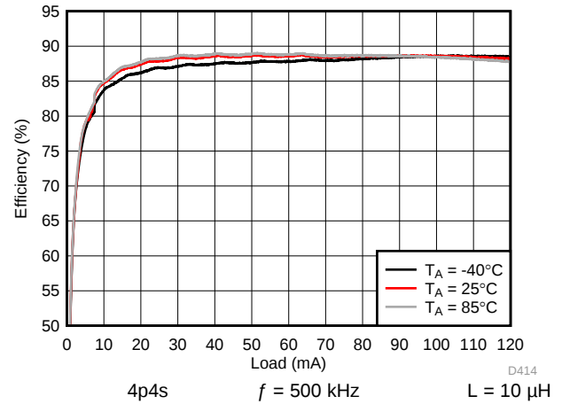
图 164. Backlight System Efficiency
