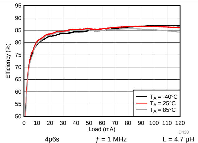
图 178. Backlight System Efficiency
