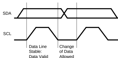
Figure 34. Bit Transfer
