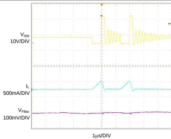
Figure 39. Steady State Operation With Light Load (200 \mu A/String, 6 Strings)
