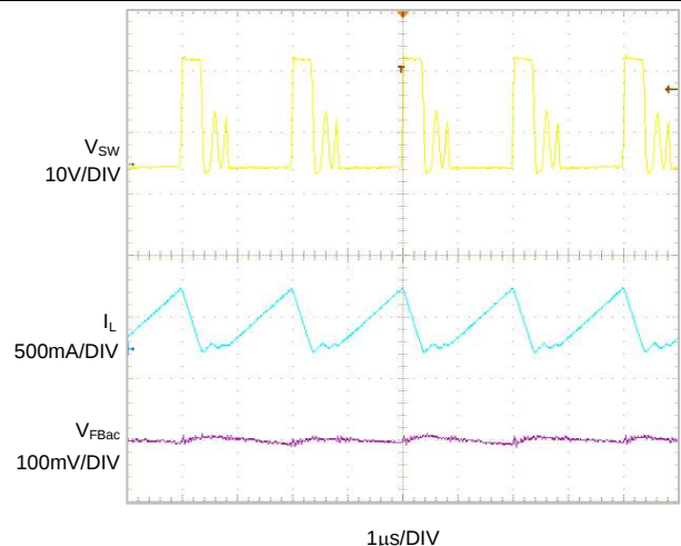
Figure 40. Steady State Operation With Medium Load (5 mA/String, 6 Strings)
