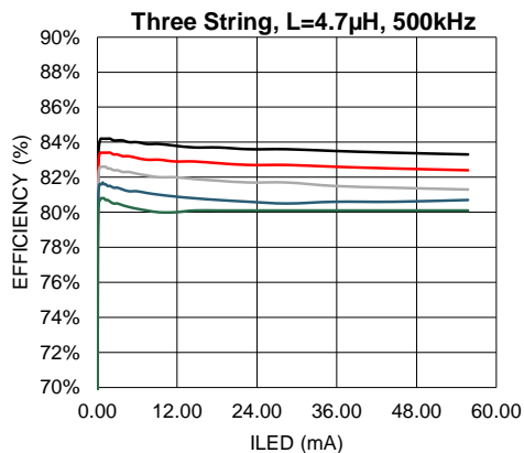
Figure 40. Boost Efficiency vs I_{LED}
