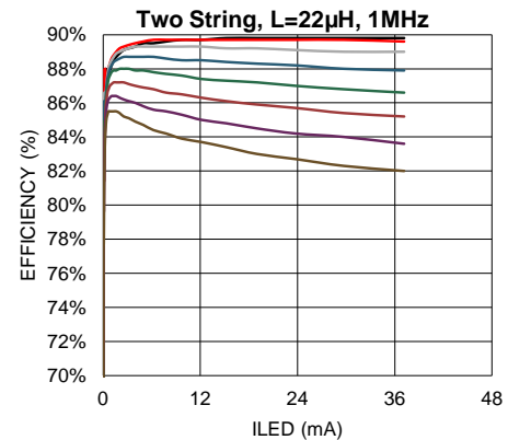
Figure 35. Boost Efficiency vs I_{LED}
