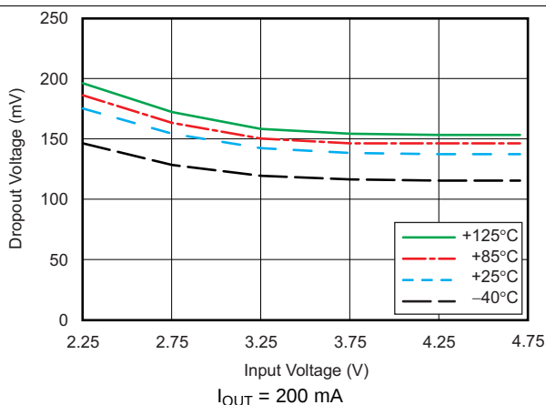
Figure 10. TLV70048-Q1 Dropout Voltage vs Input Voltage
