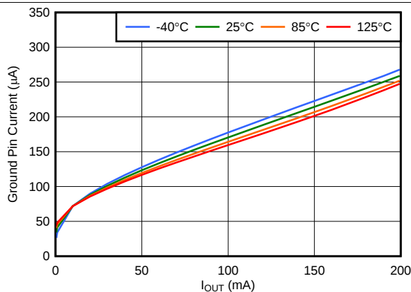
Figure 7. TLV70028-Q1 Ground Pin Current vs Output Current
