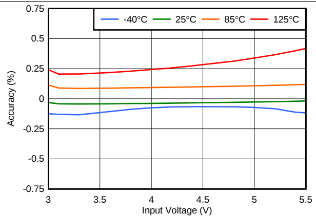
Figure 2. TLV70028-Q1 Line Regulation
