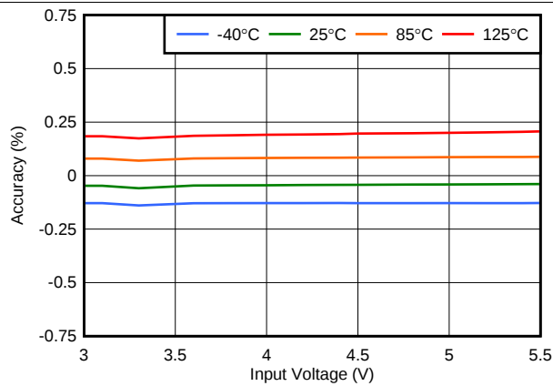
Figure 1. TLV70028-Q1 Line Regulation
