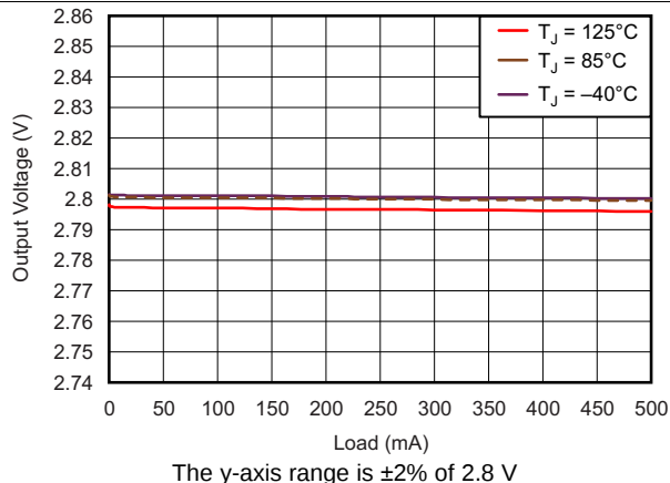
Figure 3. TPS73501-Q1 Load Regulation
