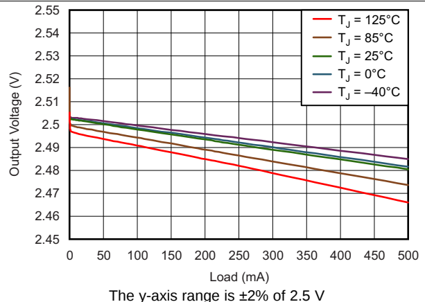
Figure 4. TPS73525-Q1 Load Regulation
