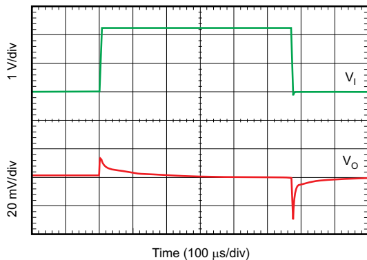
Figure 51. Line Transient Response
