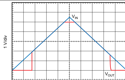
Figure 56. V_{IN} Ramp Up, Ramp Down Response
