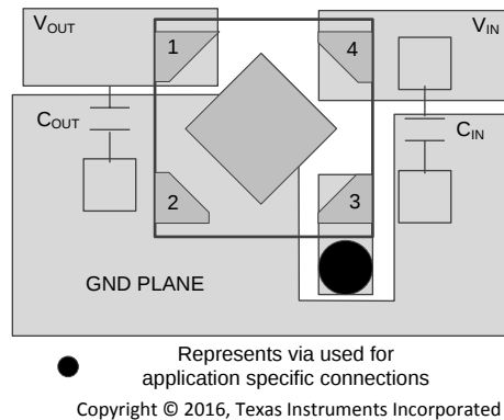
Figure 68. Recommended Layout Example
