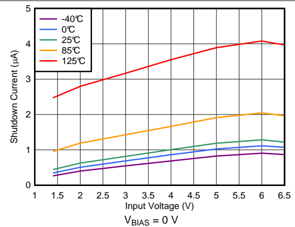
图 34. Shutdown Current vs Input Voltage
