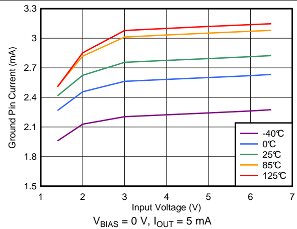
图 32. Quiescent Current vs Input Voltage
