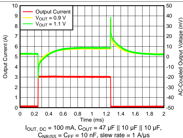
图 17. Load Transient vs Time and V_{OUT} without Bias
