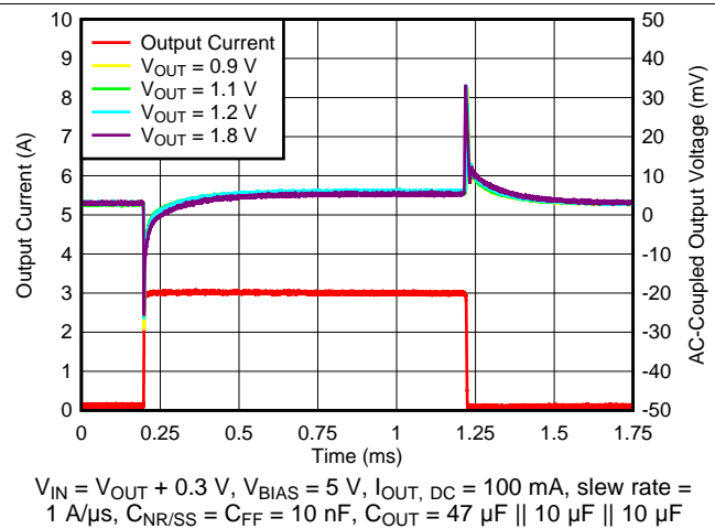
图 16. Load Transient vs Time and V_{OUT} with Bias
