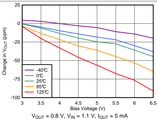
图 30. Line Regulation without Bias
