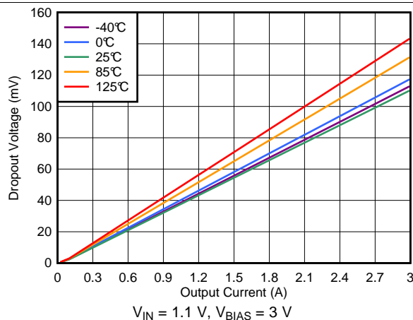
图 23. Dropout Voltage vs Output Current with Bias
