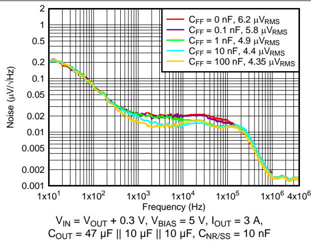
图 13. Output Noise vs Frequency and C_{FF}
