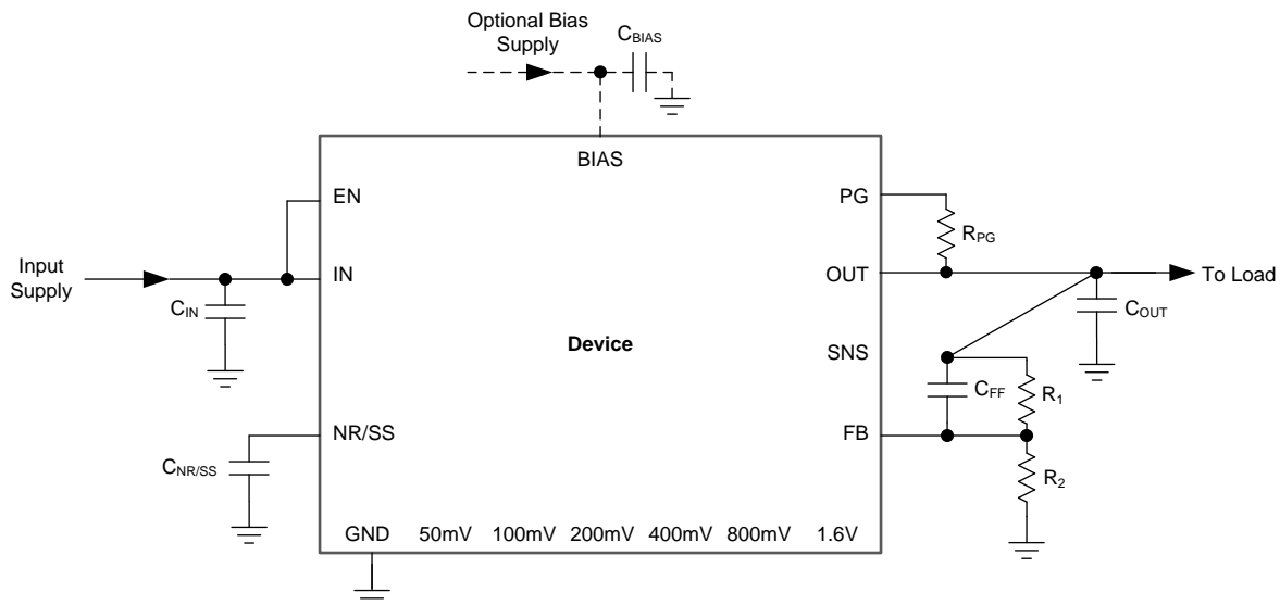
图 45. Adjustable Operation
