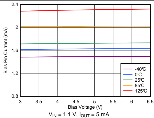
图 33. Quiescent Current vs Bias Voltage
