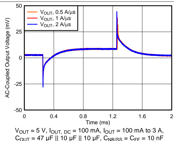
图 18. Load Transient vs Time and Slew Rate
