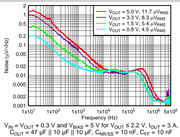
图 10. Output Noise vs Frequency and Output Voltage
