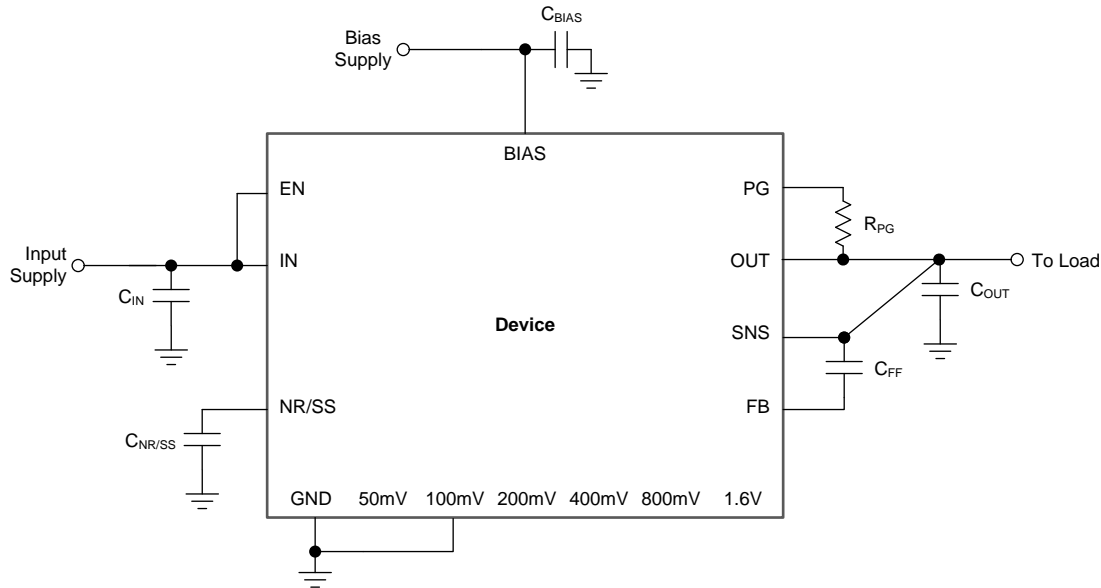
图 51. Typical Application
