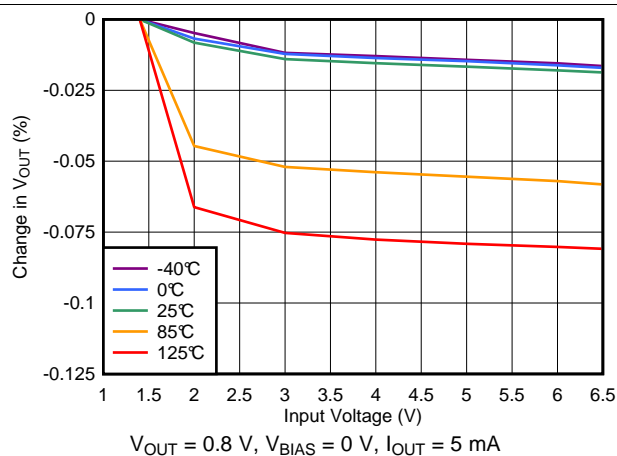
图 29. Line Regulation without Bias
