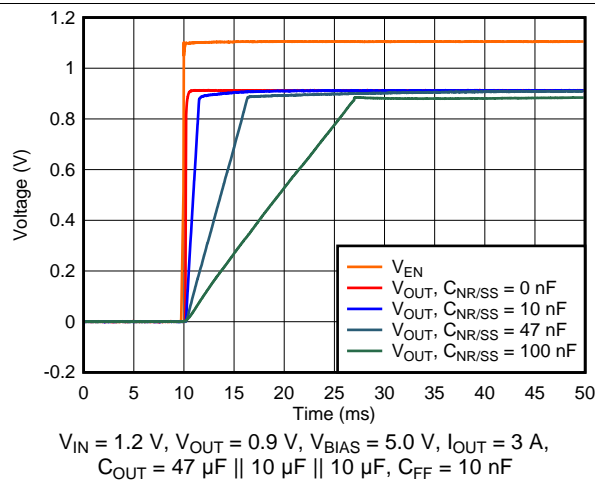
图 15. Start-Up Waveform vs Time and C_{NR/SS}
