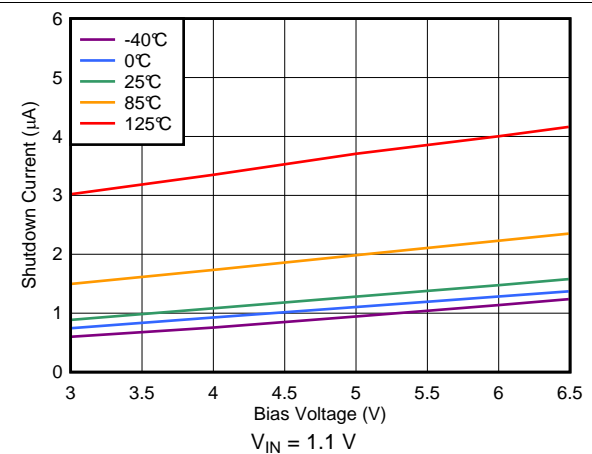
图 35. Shutdown Current vs Bias Voltage
