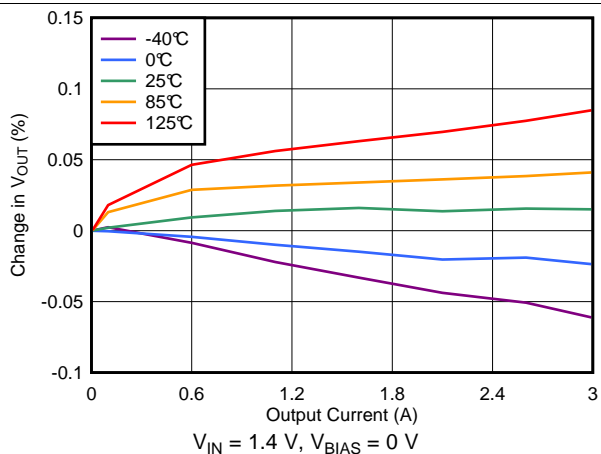
图 26. Load Regulation with Bias
