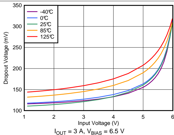
图 21. Dropout Voltage vs Input Voltage with Bias
