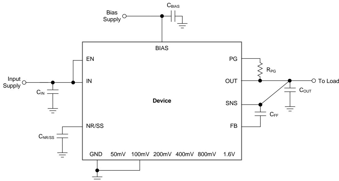
图 44. ANY-OUT Configuration Circuit (0.9-V Output with Bias)
