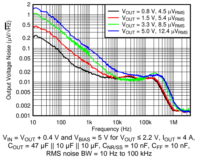
图 10. Output Noise vs Frequency and V_{OUT}
