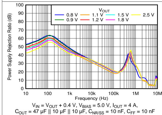
图 5. PSRR vs Frequency and V_{OUT} With Bias
