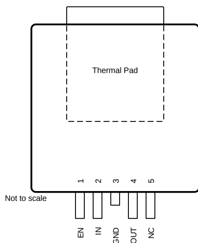
Figure 5-3. KVV Package (Fixed), 5-Pin TO-252, Top View
