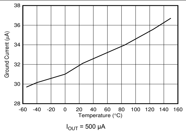
Figure 6-10. 500- \mu\text{A} Ground Current vs Temperature
