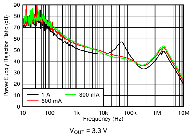
Figure 6-27. PSRR vs I_{OUT}
