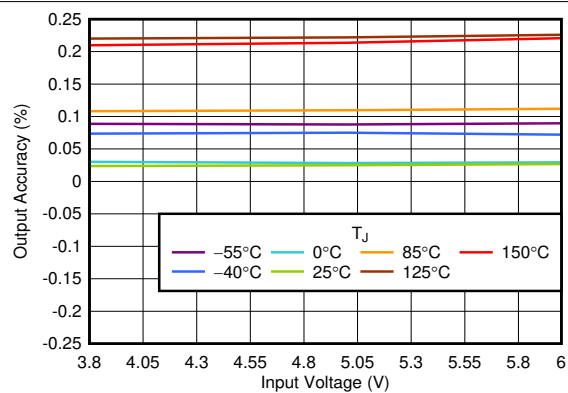
Figure 6-1. Output Accuracy vs V_{\text{IN}}
