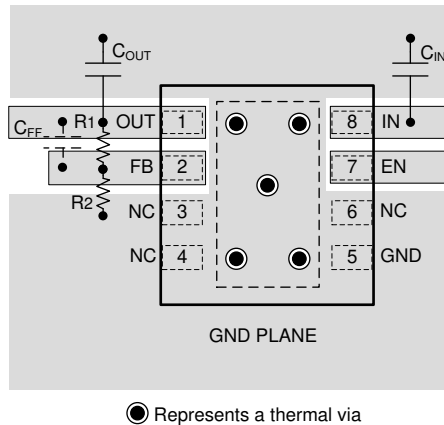
Figure 10-7. Layout Example for the DRB Package Adjustable Version
