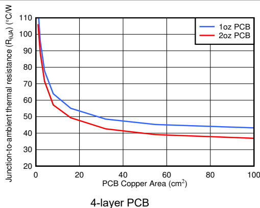
Figure 10-1. Junction-to-Ambient Thermal Resistance ( R_{JA} ) vs PCB Copper Area (DRB Package)
