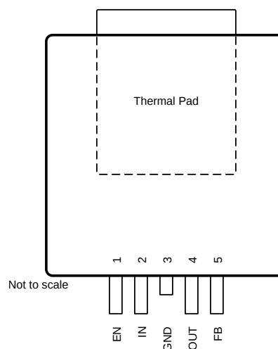
Figure 5-4. KVV Package (Adjustable), 5-Pin TO-252, Top View
