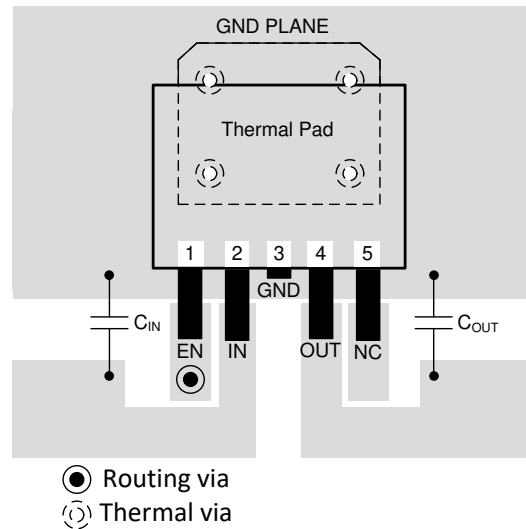
Figure 10-10. Layout Example for the KVV Package Fixed Version
