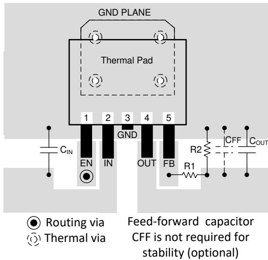
Figure 10-9. Layout Example for the KVV Package Adjustable Version
