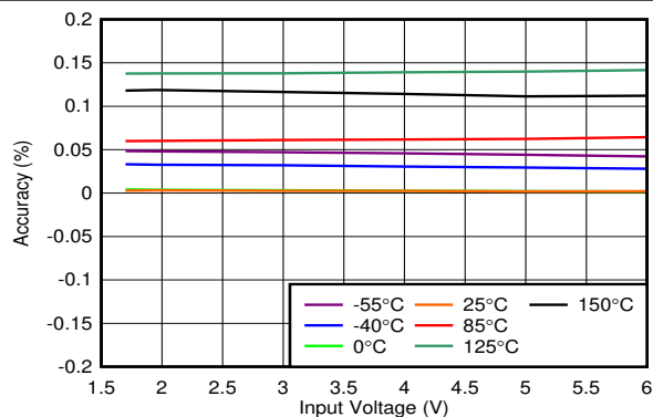
Figure 6-1. Output Accuracy vs V_{\text{IN}}
