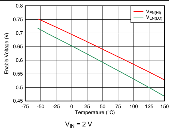
Figure 6-14. V_{EN(HI)} and V_{EN(LO)} Thresholds vs Temperature
