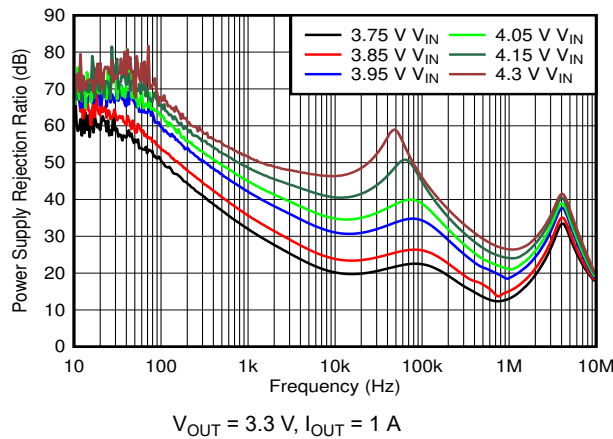
Figure 6-25. PSRR vs V_{IN}
