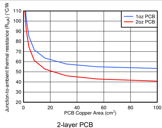
Figure 10-2. Junction-to-Ambient Thermal Resistance ( R_{JA} ) vs PCB Copper Area (DRB Package)
