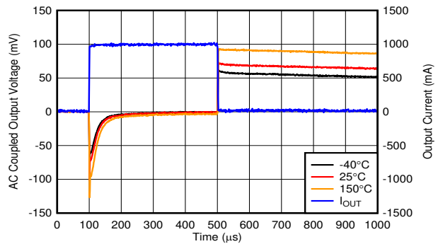
Figure 6-20. Load Transient vs Temperature
