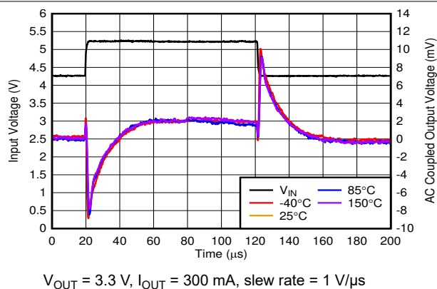
Figure 6-17. Line Transient vs Temperature
