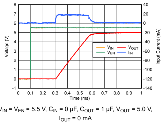
Figure 6-32. Start-Up Inrush Current With C_{OUT} = 1\text{ }\mu\text{F}
