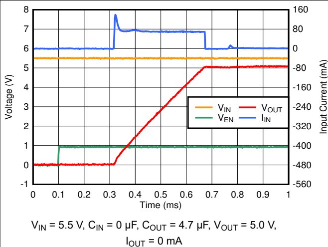
Figure 6-33. Start-Up Inrush Current With C_{OUT} = 4.7\text{ }\mu\text{F}
