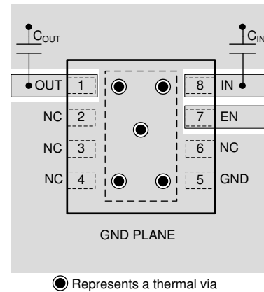
Figure 10-8. Layout Example for the DRB Package Fixed Version
