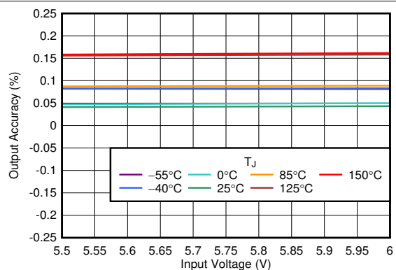
Figure 6-2. Output Accuracy vs V_{\text{IN}}
