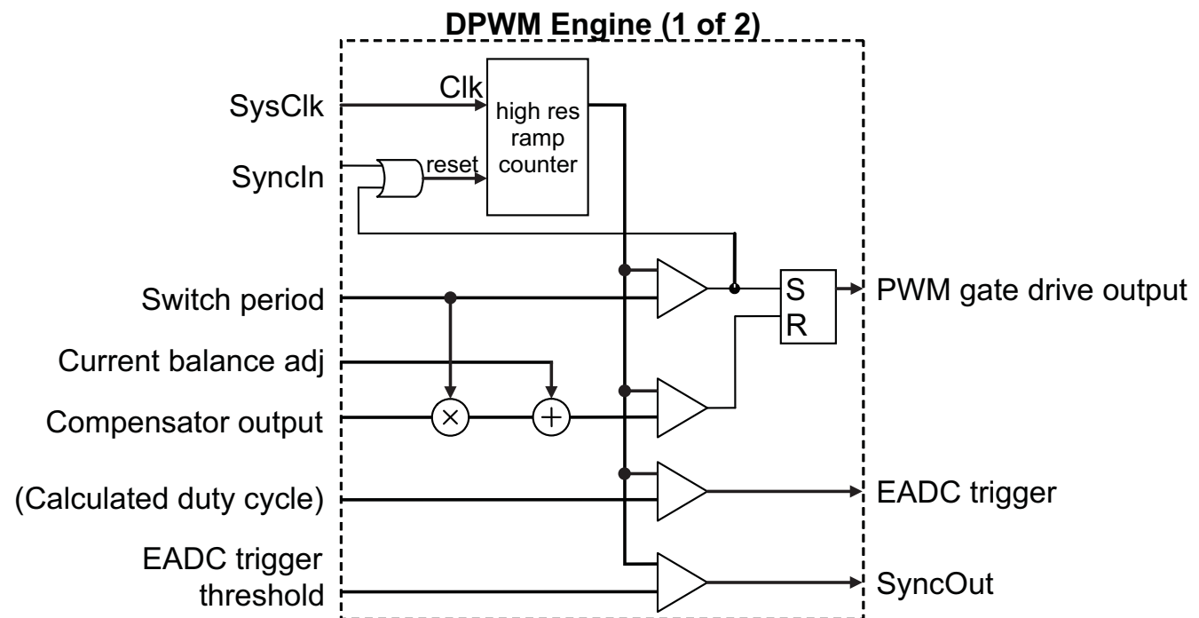
Figure 14. DPWM Engine
