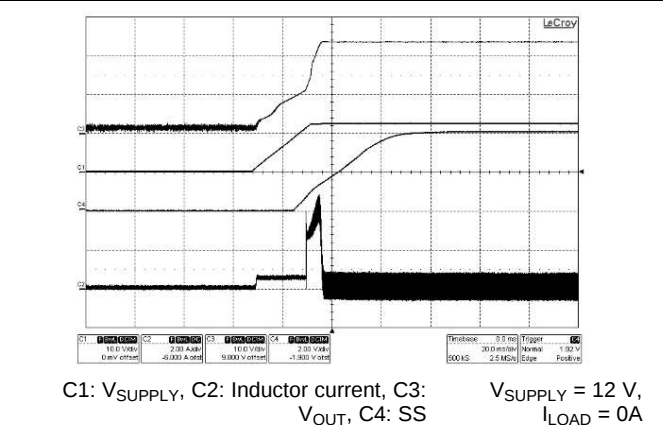
Figure 47. Start-Up
