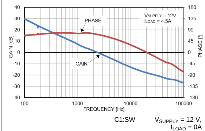
Figure 46. Loop Response
