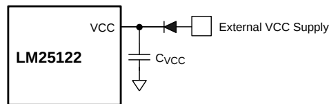
Figure 17. External Bias Supply when 9 V < V_{\text{EXT}} < 14.5 V
