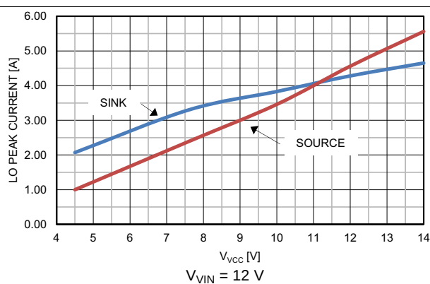
Figure 2. LO Peak Current vs V_{VCC}
