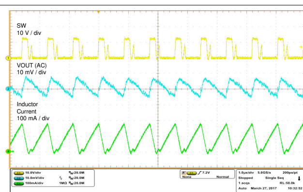
图 8-3. Switching Waveforms in PWM DCM Mode
