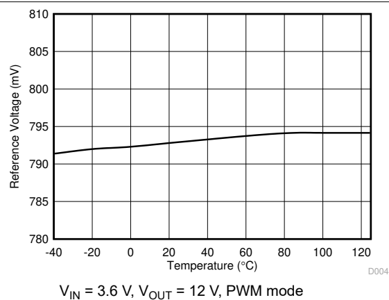
图 6-4. FB Reference Voltage vs Temperature
