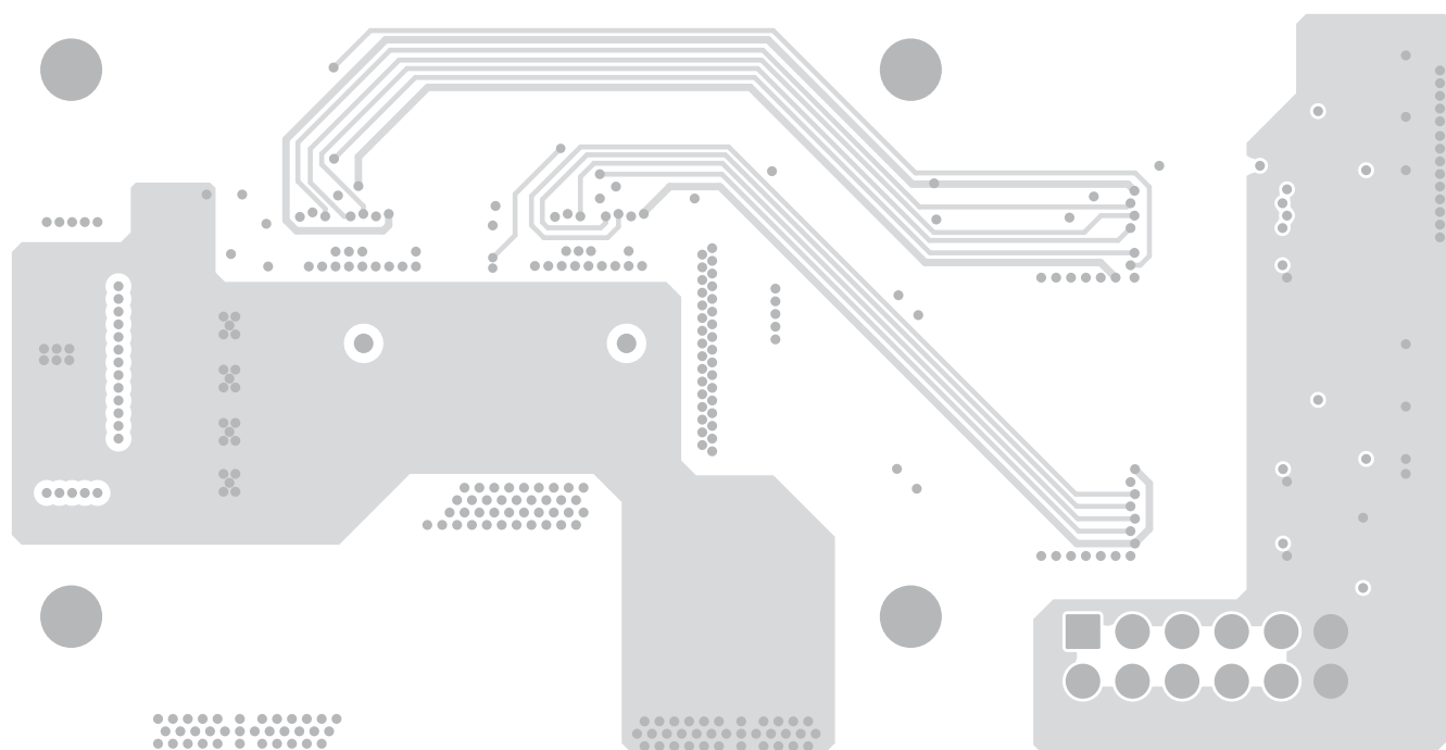
Figure 12-2. Half-Bridge Second Layer Layout
