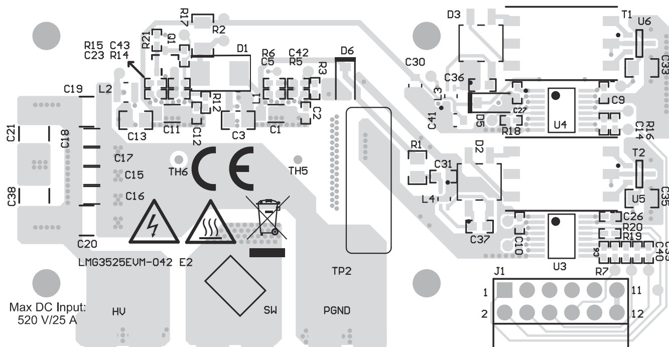
Figure 12-1. Half-Bridge Top Layer Layout
