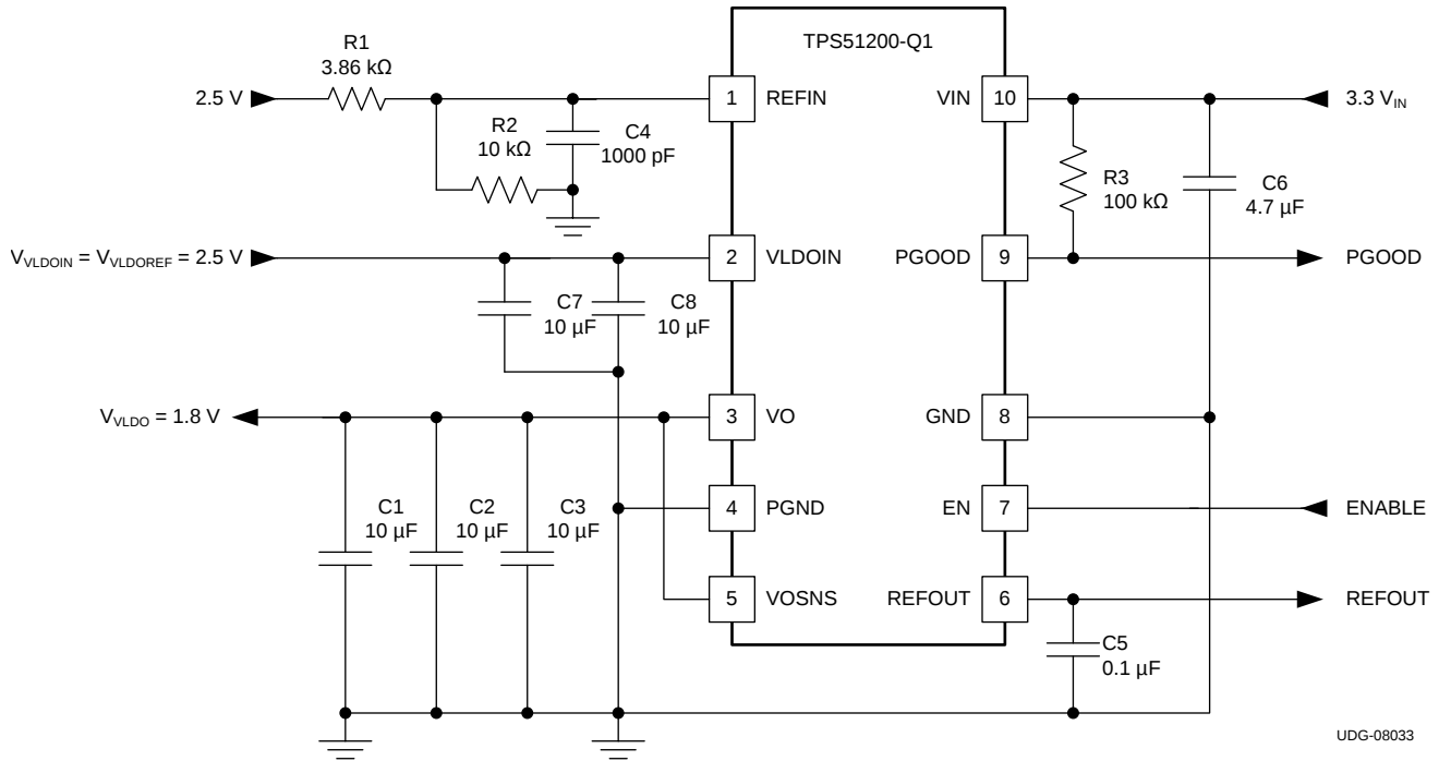
图 31. 3.3\text{-V}_{\text{IN}} , LDO Configuration
