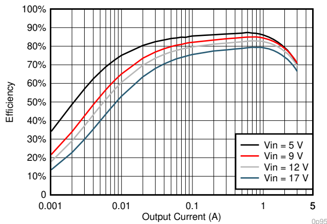
Figure 6-9. V_{OUT} = 0.95 V Efficiency, L = 1.2 \mu H
