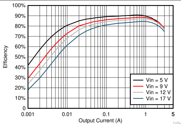
Figure 6-11. V_{OUT} = 1.5 V Efficiency, L = 1.5 \mu H
