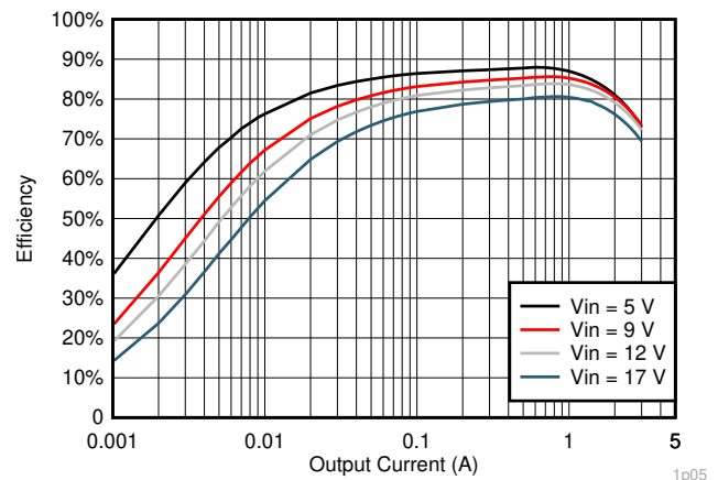
Figure 6-10. V_{OUT} = 1.05 V Efficiency, L = 1.2 \mu H
