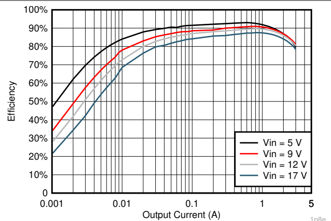
Figure 6-12. V_{OUT} = 1.8 V Efficiency, L = 2.2 \mu H
