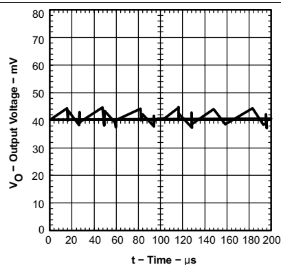
Figure 16. Output Ripple Voltage
