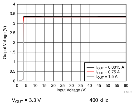
Figure 10-9. Line Regulation
