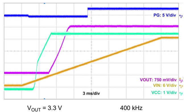
Figure 10-15. Start-Up Waveform
