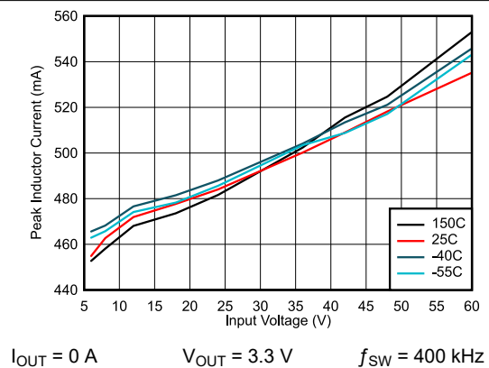
Figure 8-6. I_{PEAK-MIN}
