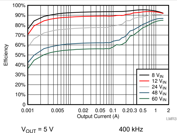
Figure 10-4. Efficiency
