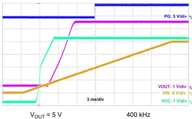
Figure 10-14. Start-Up Waveform
