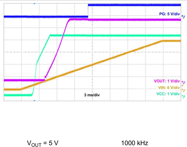
Figure 10-33. Start-Up Waveform
