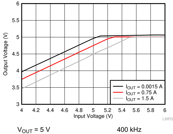
Figure 10-10. Overall Dropout Characteristic
