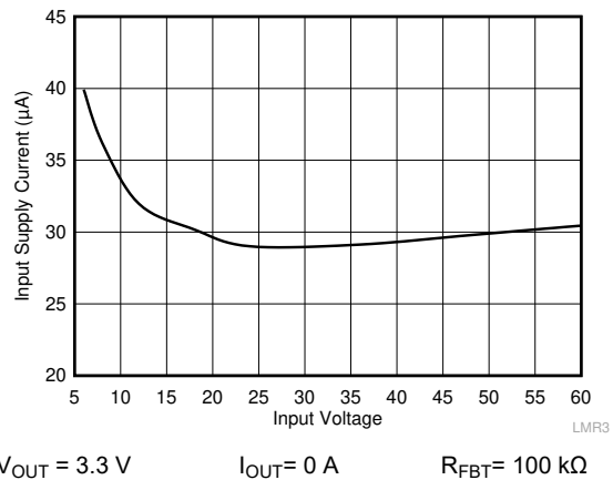
Figure 10-12. Input Supply Current
