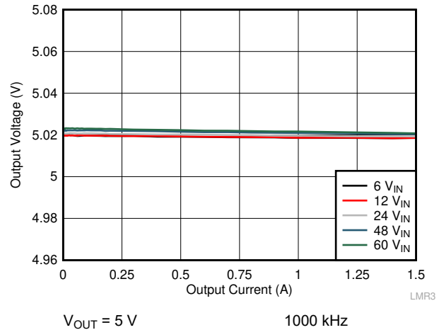
Figure 10-29. Load Regulation
