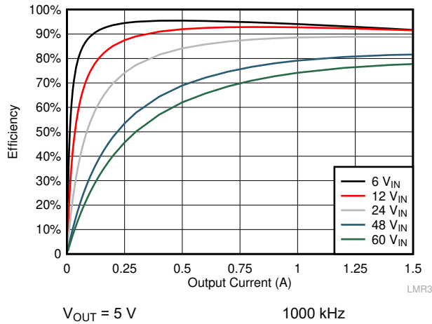
Figure 10-28. Efficiency
