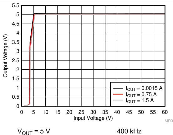
Figure 10-8. Line Regulation
