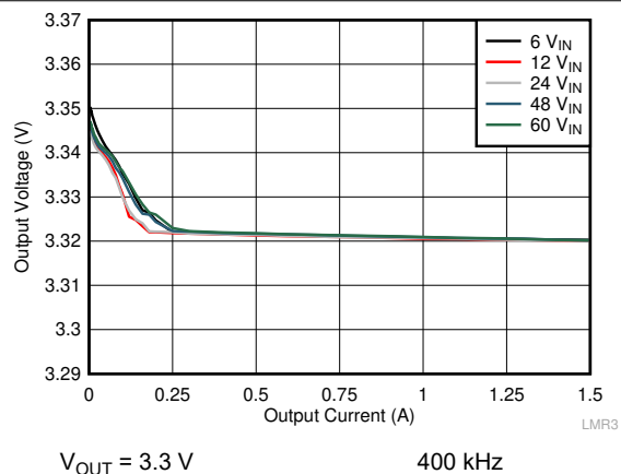
Figure 10-7. Load Regulation
