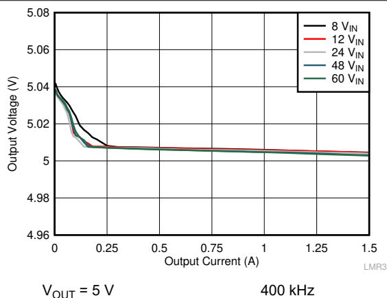
Figure 10-6. Load Regulation
