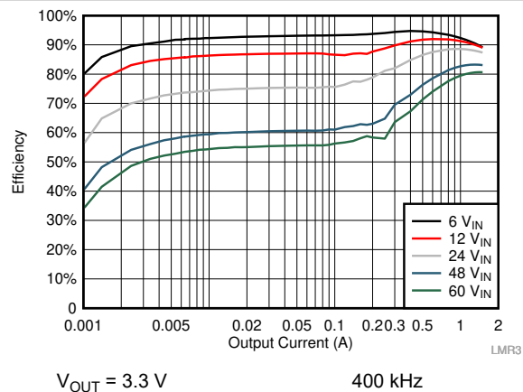
Figure 10-5. Efficiency
