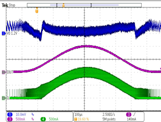
TPS62801 V_{OUT} = 1.2\text{ V} VSEL/MODE = GND I_{OUT} = 1\text{ mA to }1\text{ A }1\text{ kHz} PFM/PWM Mode
