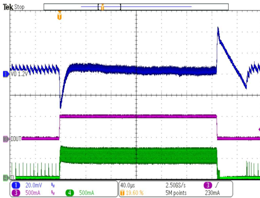
TPS62801 V_{OUT} = 1.2\text{ V} VSEL/MODE = GND rise / fall time < 1\text{ }\mu\text{s} PFM / PWM Mode I_{OUT} = 5\text{ mA to }500\text{ mA}
