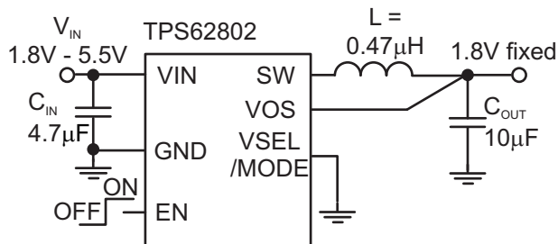
图 60. TPS62802 VSEL Connected to GND for 1.8V Fixed V_{OUT}
