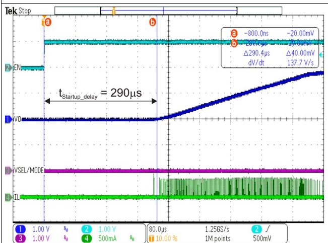
VSEL/MODE = \text{GND}
