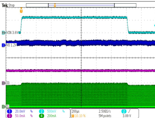
TPS62801 V_{OUT} = 1.2\text{ V} V_{IN} = 3.6\text{ V to }4.2\text{ V} rise / fall time = 10\text{ }\mu\text{s} I_{OUT} = 50\text{ mA}
