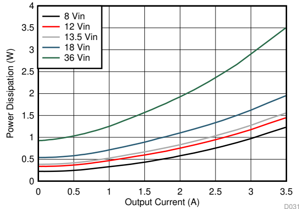
Figure 22. Power Dissipation 5-V Output
