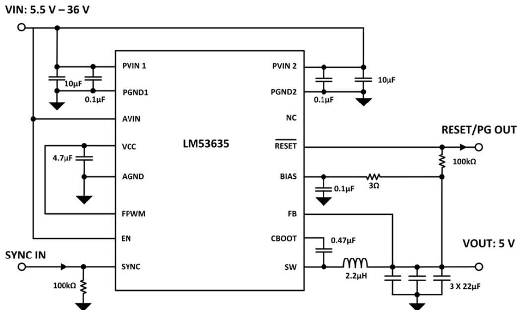
Figure 24. Fixed 5-V, 3.5-A Output Power Supply
