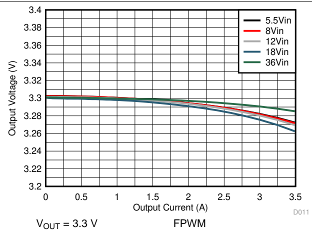
Figure 42. Load and Line Regulation
