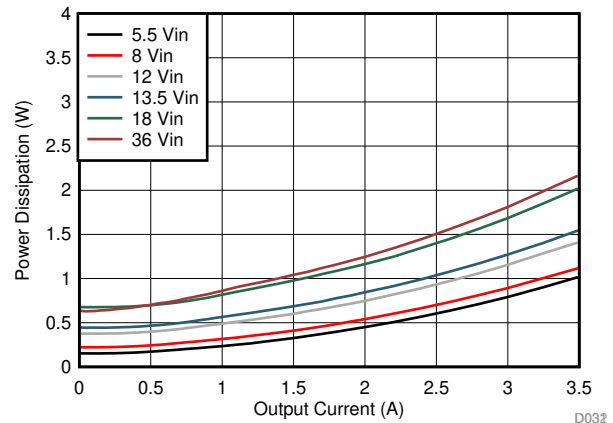
Figure 23. Power Dissipation 3.3-V Output
