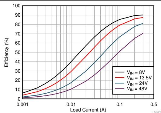
Figure 7-2. Efficiency 5-V Output, FPWM
