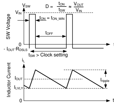
Figure 8-21. Valley Current Mode Operation
