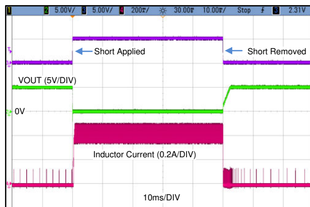
Figure 8-15. Short Circuit Waveform
