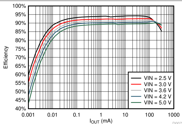
图 9-3. Efficiency vs Load Current; V_{OUT} = 2.1\text{ V}
