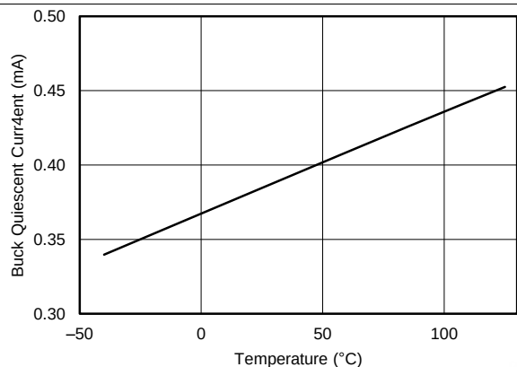
Figure 1. TPS56420 Supply Current vs Junction Temperature
