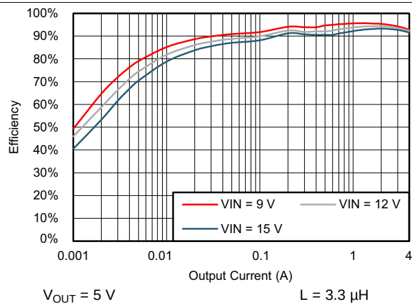
Figure 13. TPS564201 Efficiency vs Output Current
