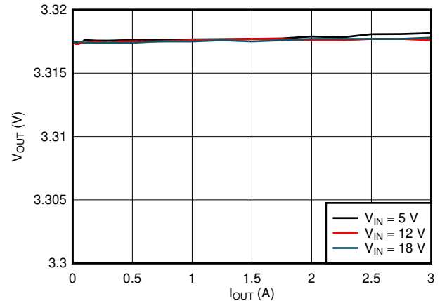
图 8-5. Load Regulation
