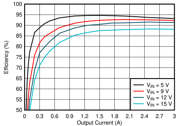
图 8-22. Efficiency
