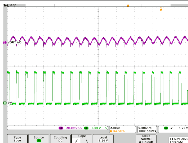
V_{IN} = 12\text{ V} I_{OUT} = 0\text{ A} 图 8-14. Output Ripple - No Load
