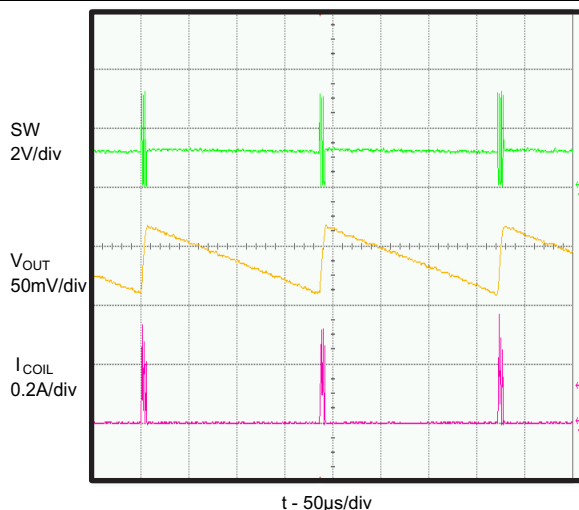
Figure 25. Typical Application (Snooze Mode)
