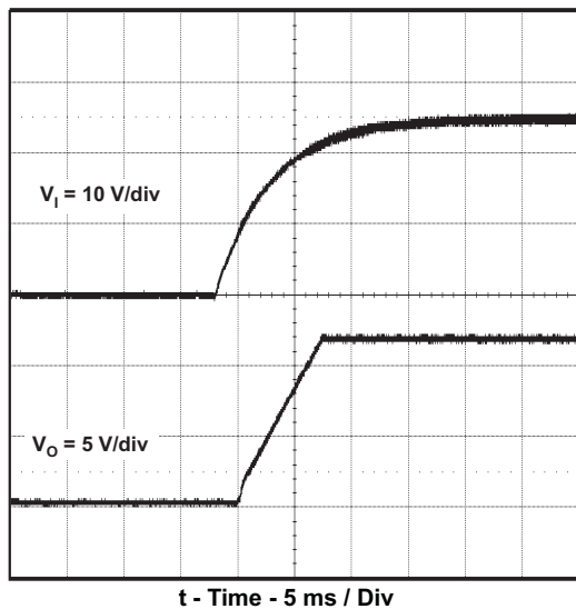
Figure 19. Startup Waveform, V_I and V_O
