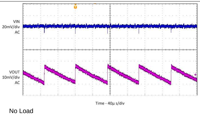
图 25. Input and Output Ripple in PSM Mode
