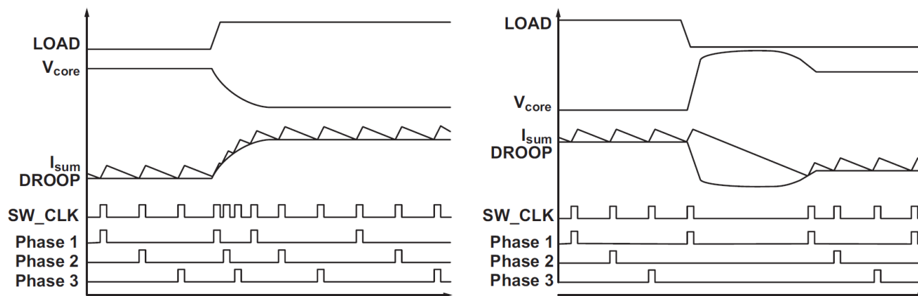
图 10. 3-Phase Transient Operation
