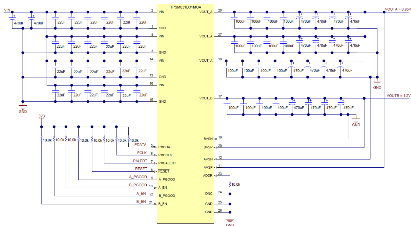
图 20. Typical Dual Output Schematic (Dual Outputs: VOUTA = 0.85 V, 120 A and VOUTB =1.2 V, 40 A)
