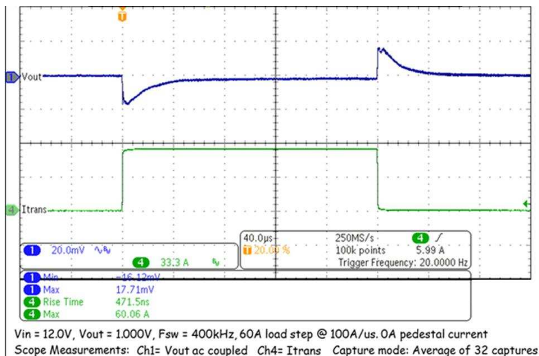
图 21. Typical Transient Response
