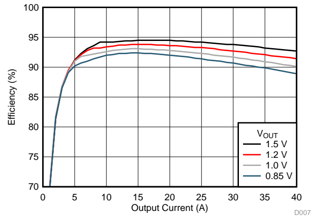
图 2. VOUTB Efficiency
