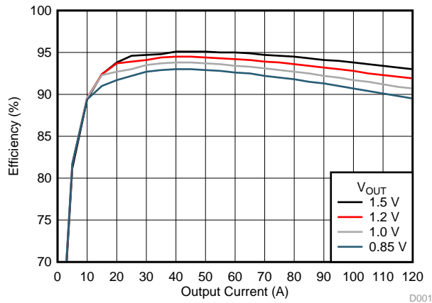
图 1. VOUTA Efficiency
