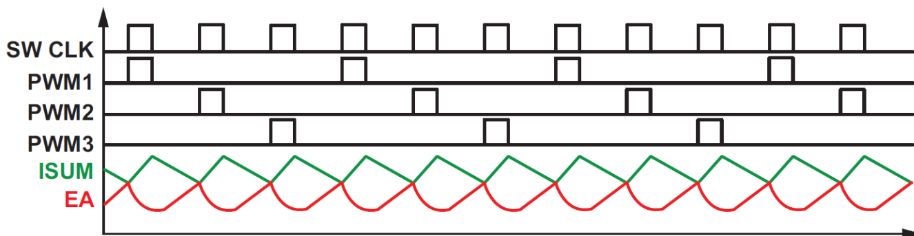
图 9. 3-Phase Steady State Switching
