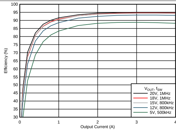
图 21. Efficiency vs Output Current
