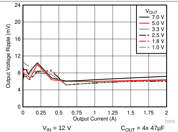
图 9. Voltage Ripple versus Output Current
