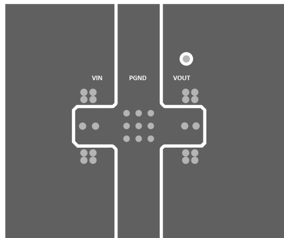
图 43. Typical Layer-2 Layout
