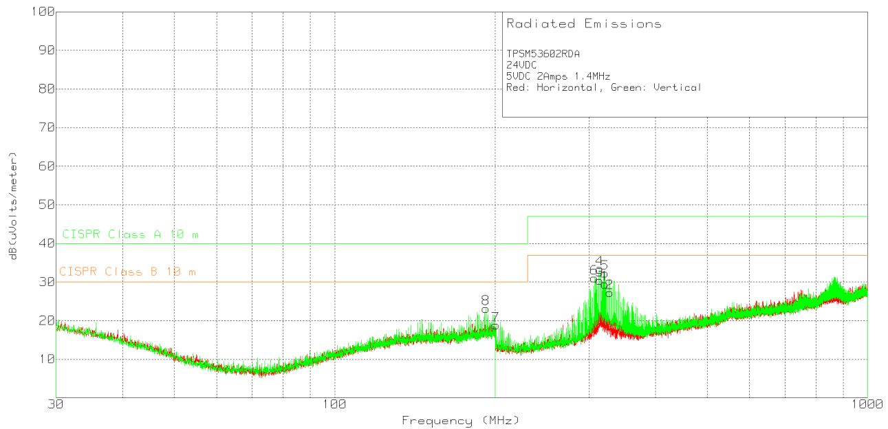
图 46. Radiated Emissions 24-V Input, 5-V Output, 2-A Load
