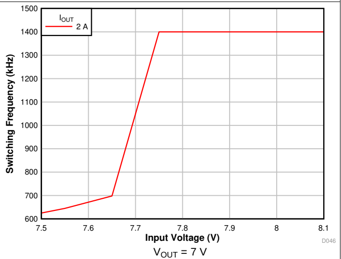
图 34. Frequency Foldback
