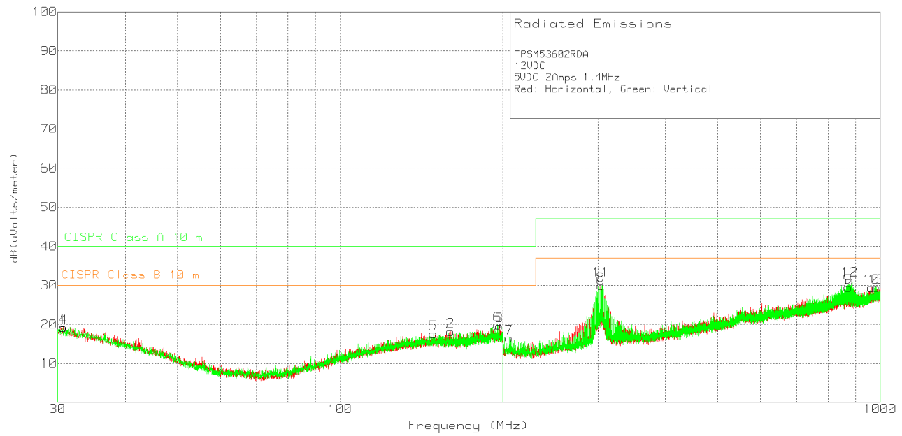
图 47. Radiated Emissions 12-V Input, 5-V Output, 2-A Load
