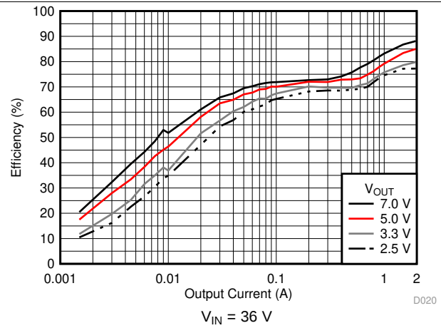
图 18. Efficiency versus Output Current
