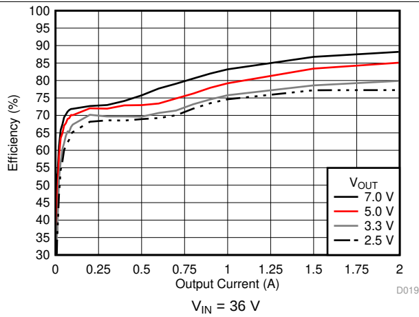
图 17. Efficiency versus Output Current
