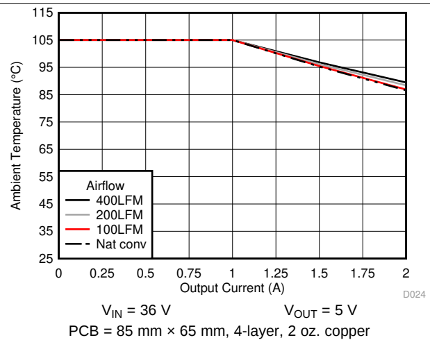
图 22. Safe Operating Area
