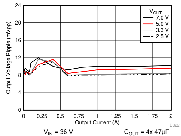
图 20. Voltage Ripple versus Output Current
