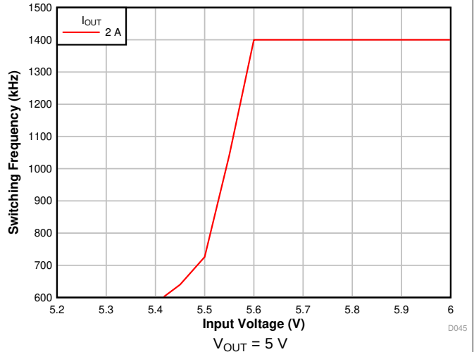
图 32. Frequency Foldback
