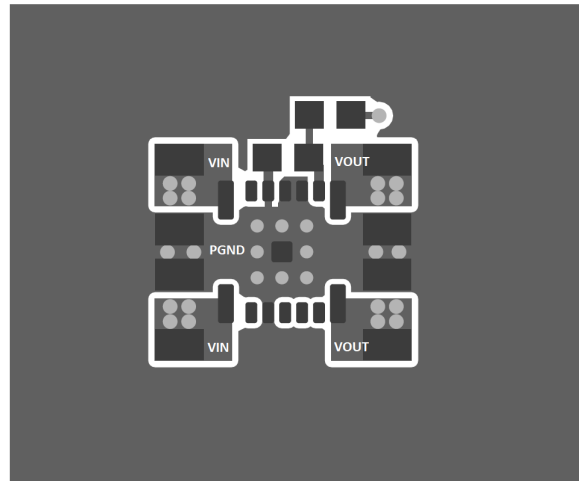
图 42. Typical Top-Layer Layout
