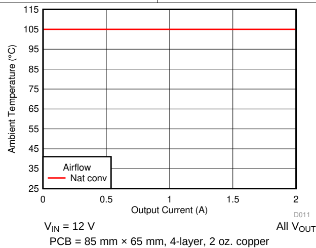
图 10. Safe Operating Area
