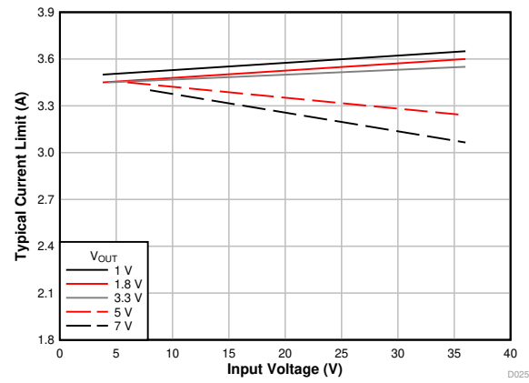
图 35. Current Limit Threshold
