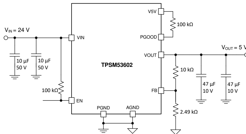
图 38. TPSM53602 Typical Schematic
